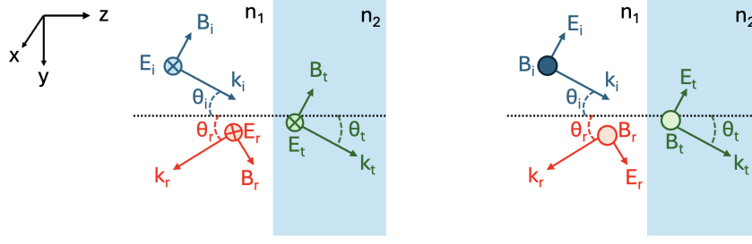
Figure 2.4: Diagram of polarized light at two interfaces. The left image shows the case for s-polarized light, with the electric field pointing into the page. For p-polarized light on the right the magnetic field points outside of the page.
