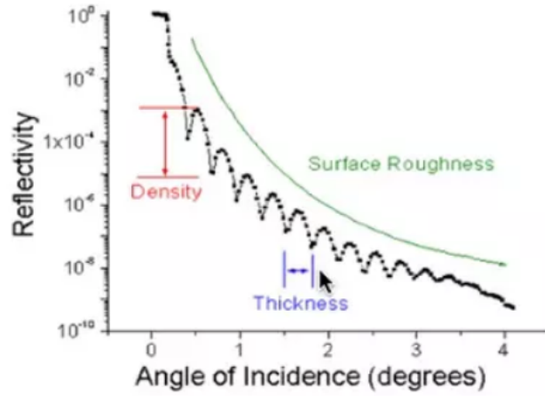
Figure 2.9: Effects of thickness, surface roughness and difference in density on the XRR intensity
