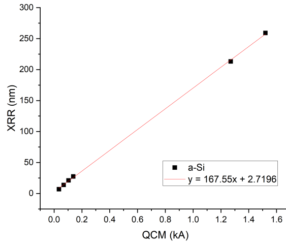
Figure 4.3: Linear regression of XRR and QCM thicknesses for a-Si thin films grown via e-beam evaporation. The high R^2 value indicates the validity of the equation in relating the QCM thickness to the actual thickness as measured by XRR.
