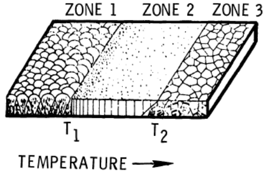
Figure 2.4: Structure zone diagram introduced by Movchan and Demchishin from study of vacuum evaporated metals and oxides.
