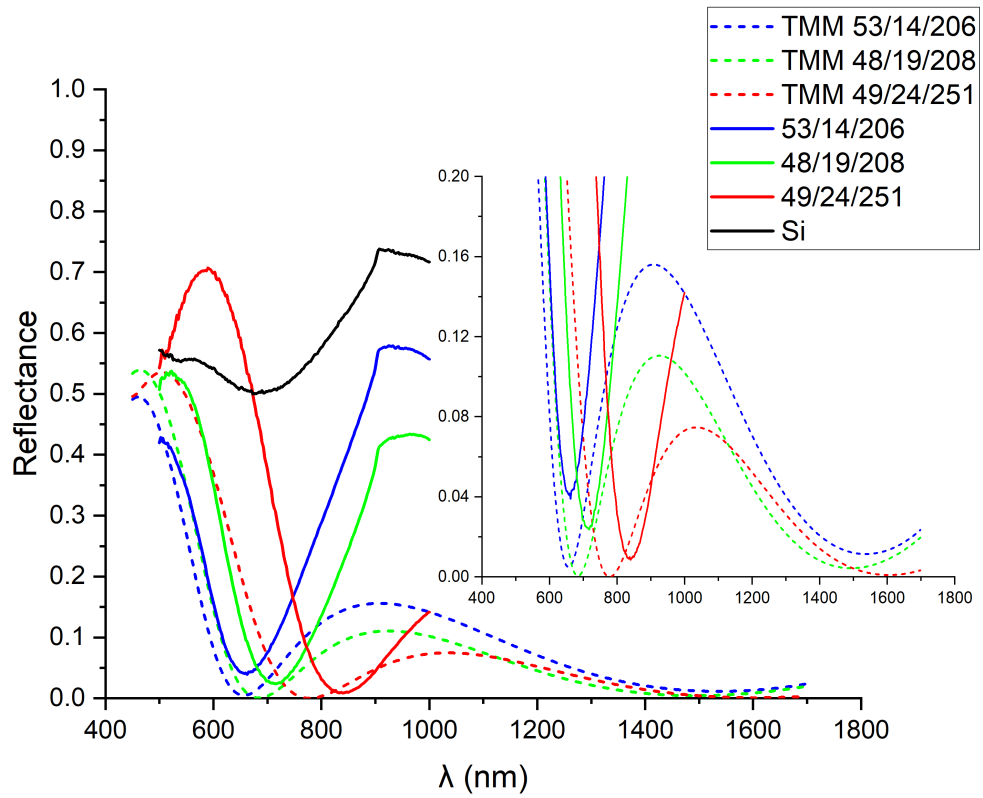
Figure 4.15: Reflectivities of antireflective coatings with varying layer thicknesses simulated using the transfer matrix method and measured experimentally. The reflectance of a bare Si wafer is included for comparison.
