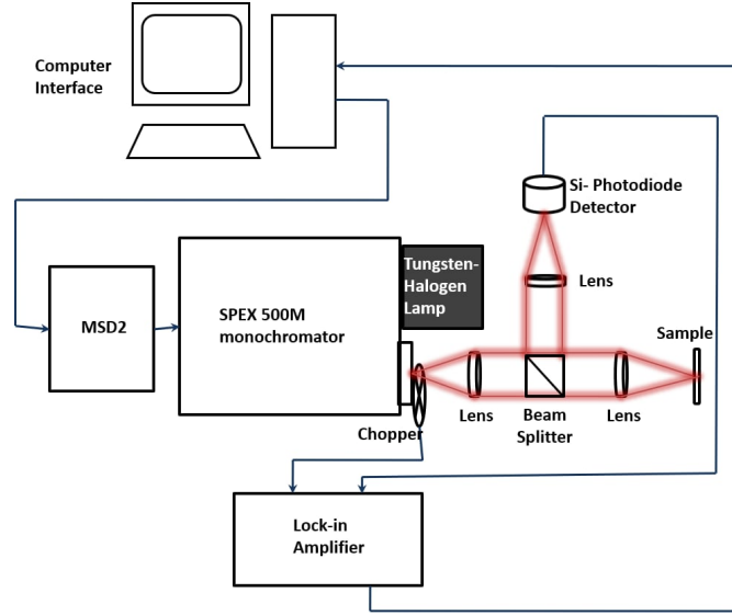
Figure 3.1: Normal incidence reflectance spectroscopy setup.
