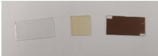
Figure 4.1: Bare glass, 0.138 kÅ and 3.050 kÅ thick a-Si films on glass. The intensity of the tint increases with the deposited a-Si thickness due to the absorption of Si in the visible range.
