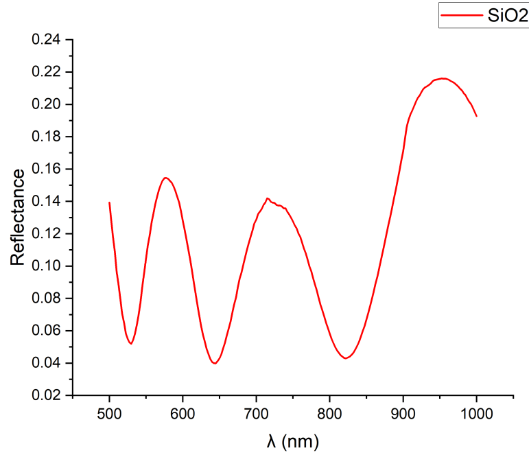
Figure 4.13: Deconvoluted reflectance spectra of 990 nm SiO 2 thin film
