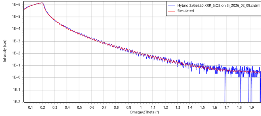
Figure 4.10: XRR curve fit to 204.7 nm SiO 2 thin film
