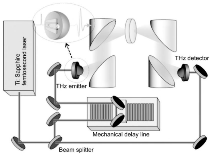
Figure 2.9: Schematic of a THz TDS setup with a femtosecond laser and two photo-conductive antennas[7]
