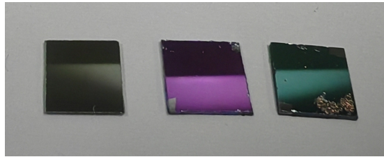
Figure 4.6: Bare Si wafer, 2.550 kÅ and 5.000 kÅ thick SiO 2 films on glass. The color of the wafer changes depending on the thickness of the deposited SiO 2 .
