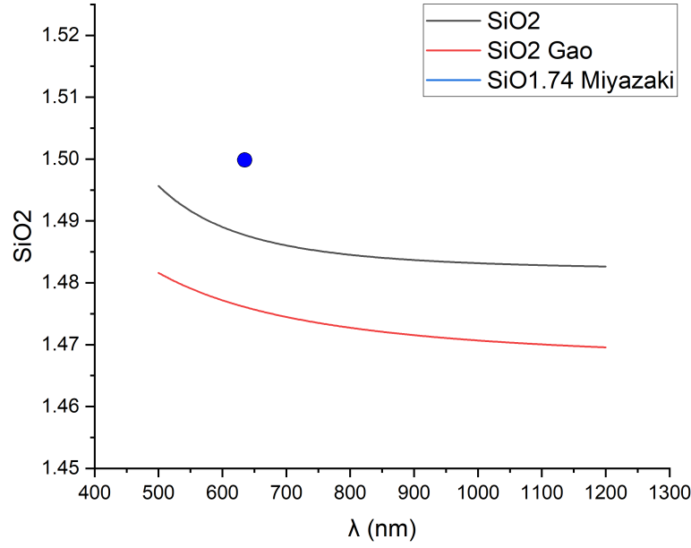
Figure 4.14: Refractive index of the SiO 2 film compared to Gao and Miyazaki
