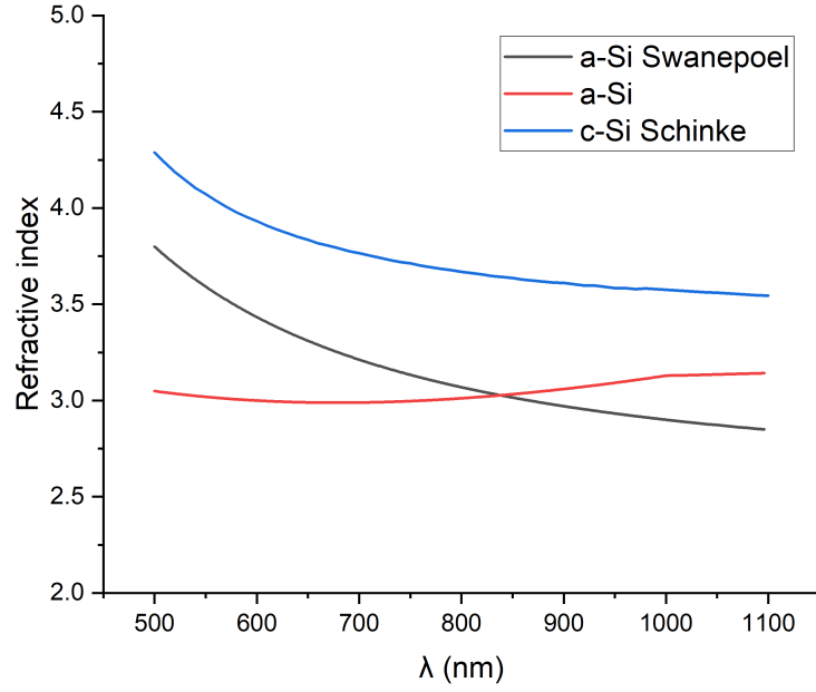
Figure 4.12: Refractive index of a-Si thin film from 500 nm to 1100 nm
