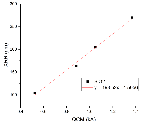
Figure 4.8: Linear regression of XRR and QCM thicknesses for SiO 2 thin films grown via e-beam evaporation.
