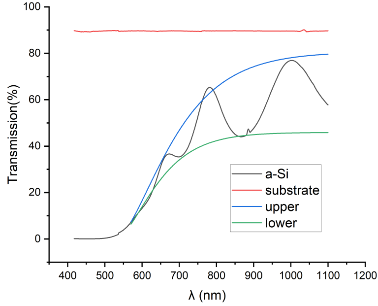
Figure 4.11: The transmission curves for the 600 nm a-Si thin film and the glass substrate together with the upper and lower envelopes for the envelope method
