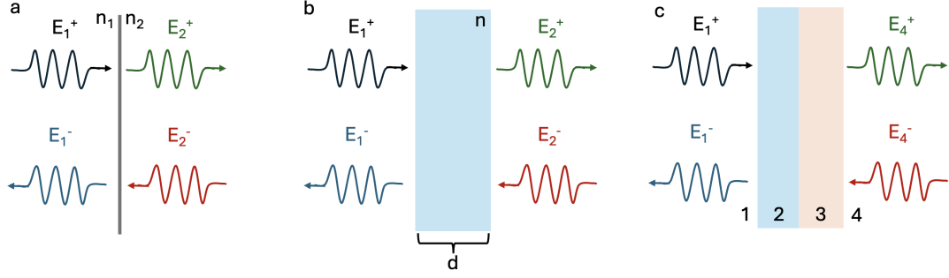
Figure 2.3: Propagation of waves at an interface (a), through a layer with refractive index n and thickness d (b), and through a multilayer system (c).
