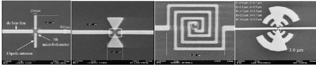
Figure 2.8: Commonly used THz PCA geometries; from left to right: dipole, bowtie, spiral, and log-spiral[45]
