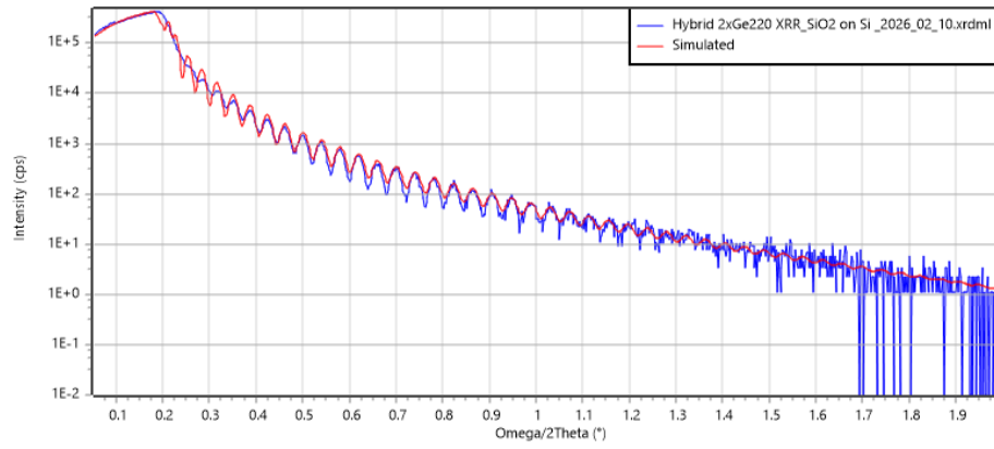
Figure 4.9: XRR curve fit to 103.9 nm SiO 2 thin film
