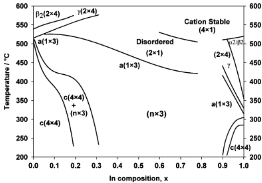
Figure 2.7: Phase diagram for the surface reconstruction of \text{In}_x\text{Ga}_{1-x}\text{As} using RHEED
