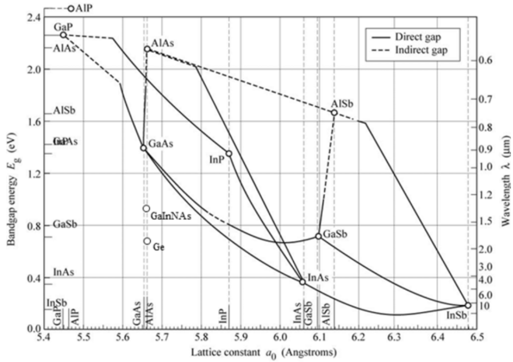
Figure 2.6: Bandgap versus lattice constant for various III-V compounds zhangBandStructureEngineering2016
