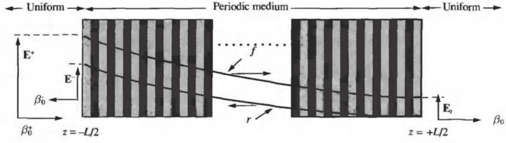
Figure 2.9: Geometry of a distributed Bragg reflector medium with a source of electromagnetic waves located on the left. The amplitude of E decreases as it propagates through the structure verdeyen Laser Electronics 2nd 1994 .
