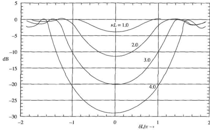
Figure 2.10: Relative power transmission of a DBR versus the detuning parameter \delta L/\pi for various coupling coefficient \kappa L values songHandbookTerahertzTechnologies2015
