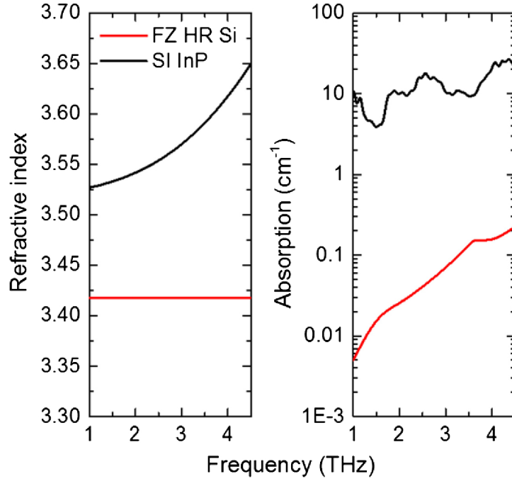
Figure 2.8: Refractive index and absorption coefficient of semi-insulating InP and float zone high resistivity Si in the THz rangesongHandbookTerahertzTechnologies2015
