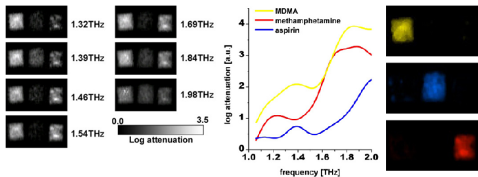
Figure 2.1: THz identification of MDMA, methamphetamine, and aspirin through a paper envelope. The substances are differentiated using their THz spectra.
