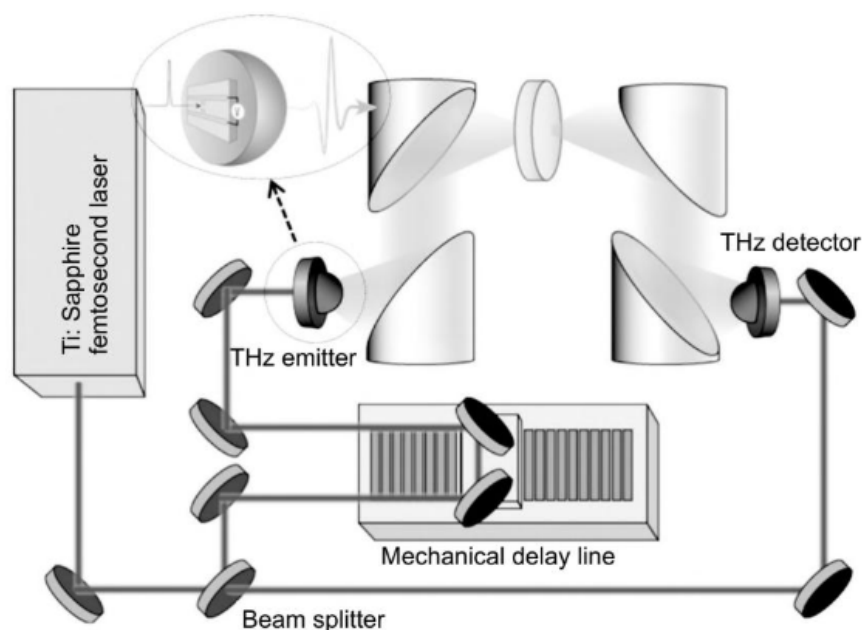
Figure 2.3: Schematic of a THz TDS setup with a femtosecond laser and two photoconductive antennas Handbook Terahertz Technologies 2015
