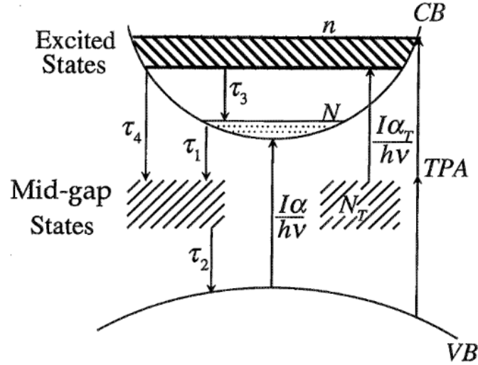
Figure 2.5: Energy level diagram of the defect states in LT-GaAs benjamin Tailoring Low temperature MBE grown 1996
