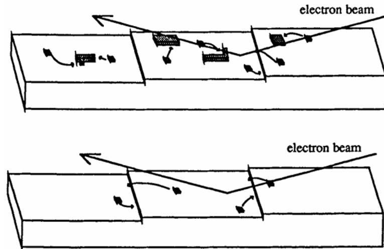
Figure 2.4: Kinetics of epitaxial growth observed using an electron beam. Molecules can form islands, migrate to step edges, or desorb from the surface. larkins2MolecularBeam1995
