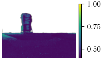
Dense Loss
