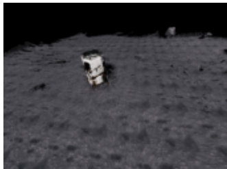
RGB (3DGS)
