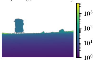
Depth (3DGS)
