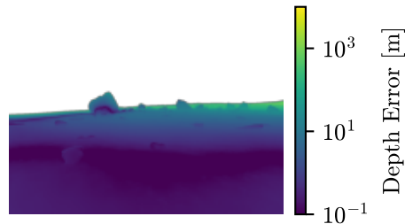
GLPN
