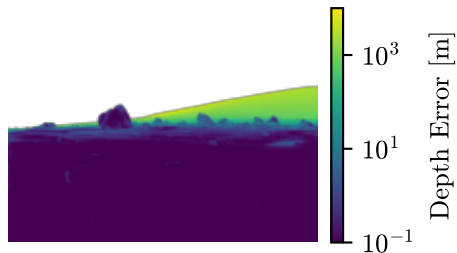
CREStereo
