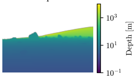
Depth
