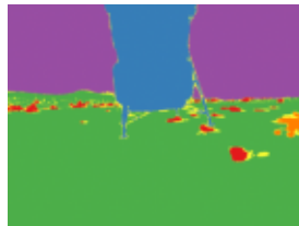
PSPNet
