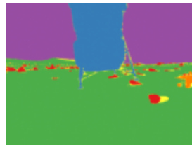
Linknet
