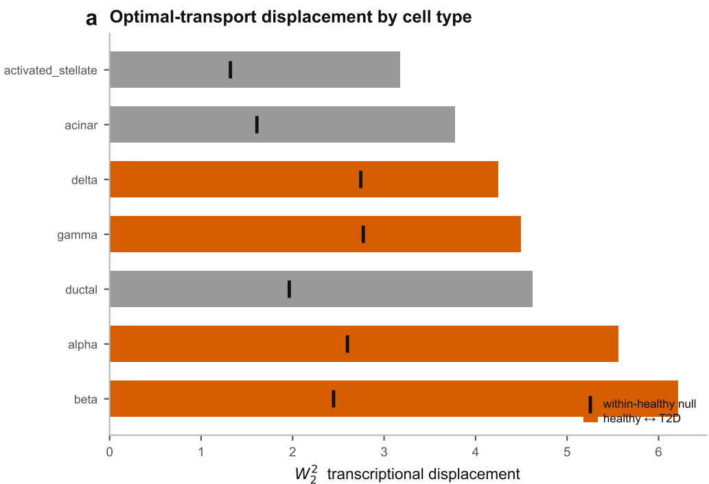
Figure 10 · Optimal transport quantifies the transcriptional displacement of diabetes
