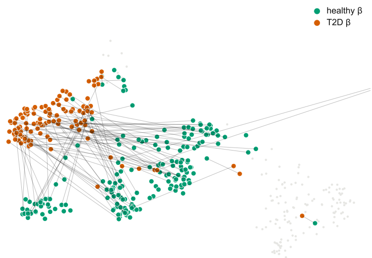
c \beta -cell transport map: healthy \rightarrow T2D
