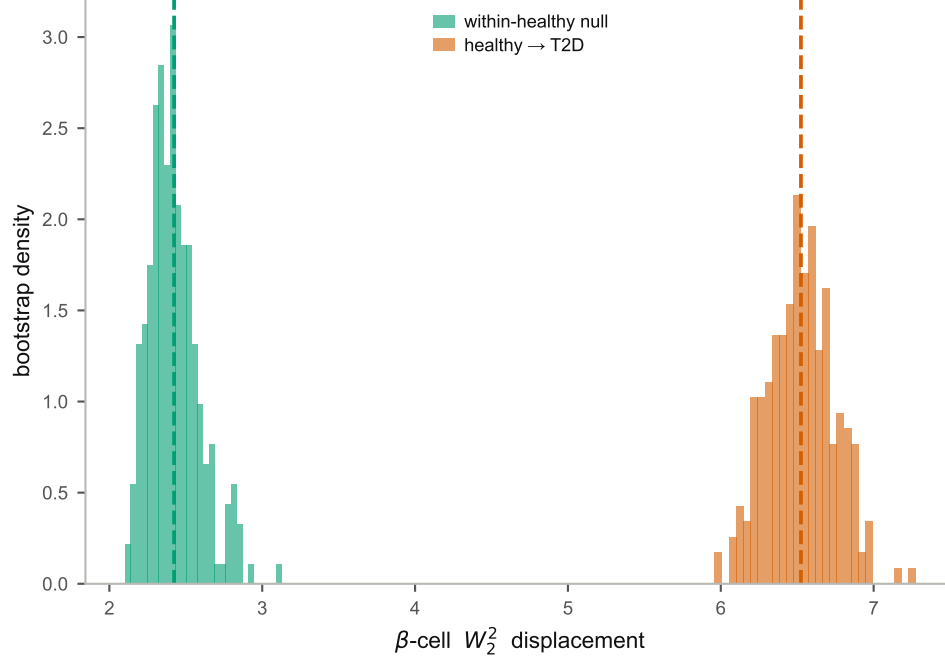
d \beta -cell shift is real: 2.7 \times null ( p < 0.004 , 250 bootstraps)
