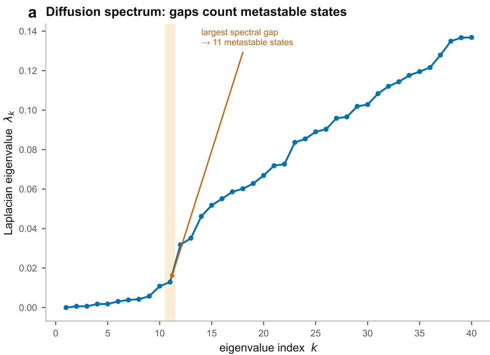
Figure 11 · Spectral & diffusion geometry with a random-matrix null
