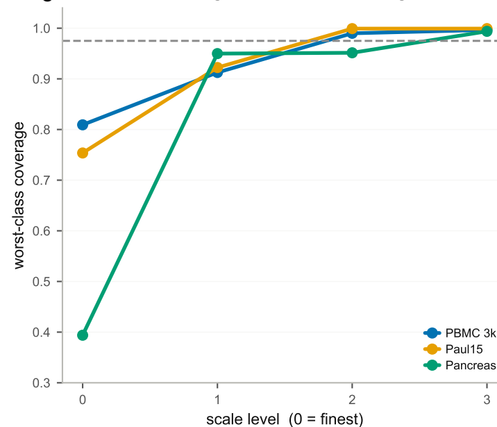
e Rare-type rescue generalizes: worst-class coverage rises with coarsening
