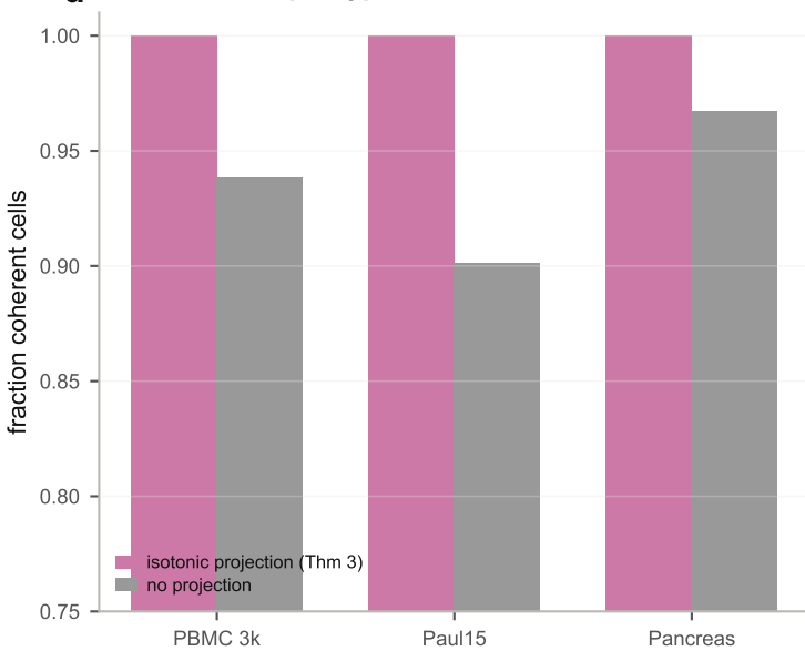
d Coherence: fine calls never contradict their coarse super-type
