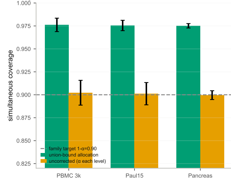
c Family-wise guarantee: the allocation buys a safety margin
