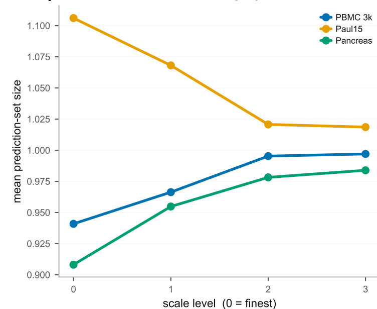
f Sets stay compact; the continuum (Paul15) carries the most residual ambiguity
