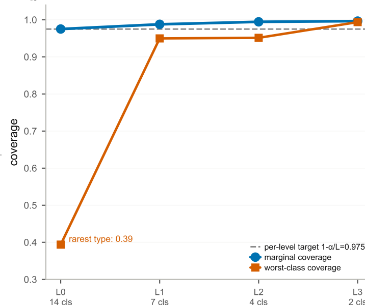
b Per-scale coverage holds; a rare type under-served at fine scale is rescued coarse
