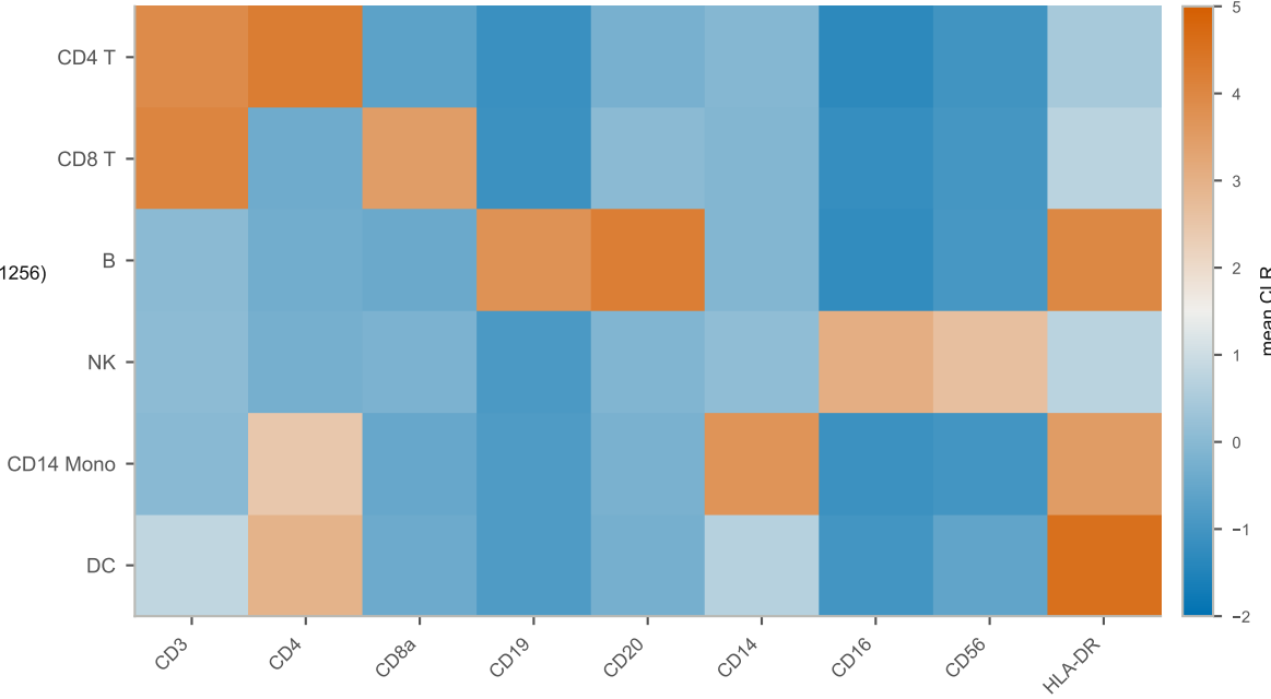
b Protein markers define the labels (independent of RNA)
