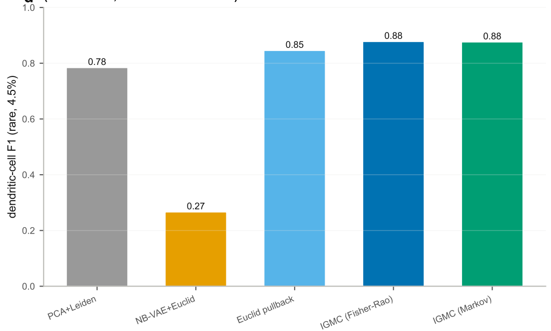
d Fisher-Rao best recovers the rare DC type (same latent, Euclidean ruler fails)
