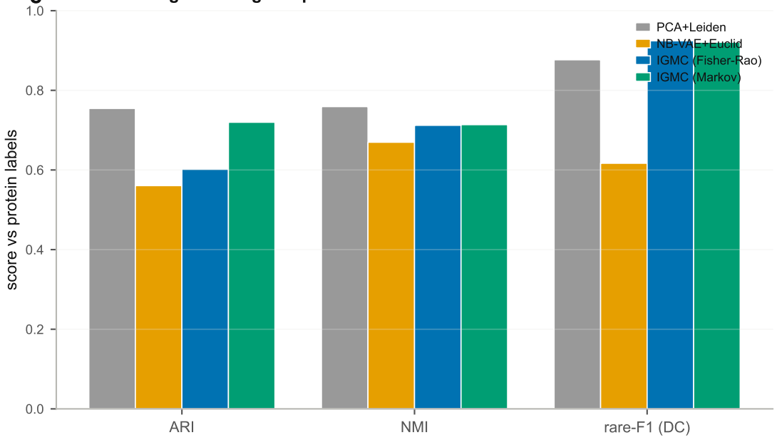
c RNA clustering vs orthogonal protein truth
