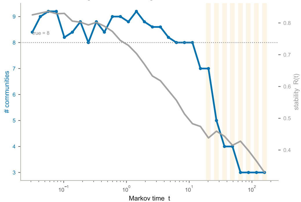
a Communities emerge as the walk lengthens
