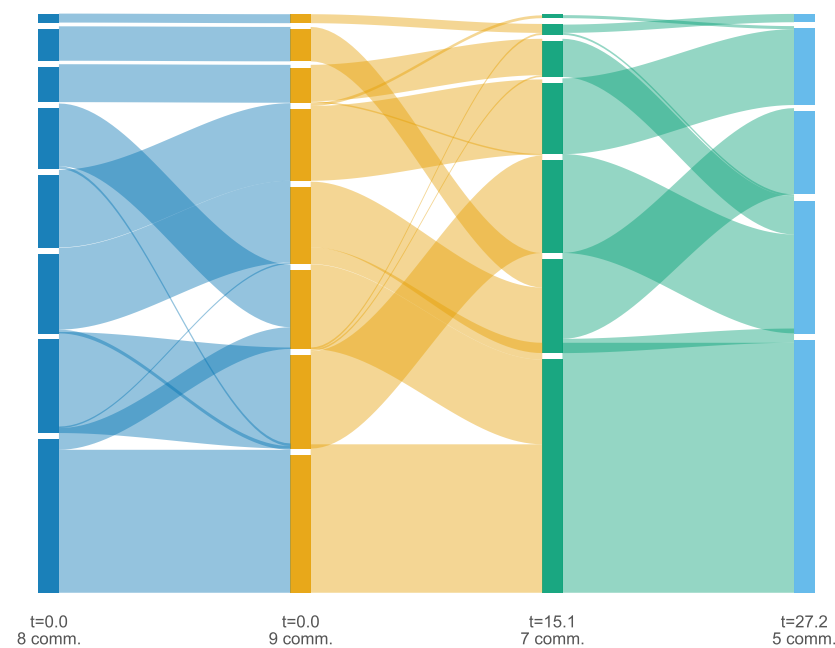
d Cluster hierarchy across scales
