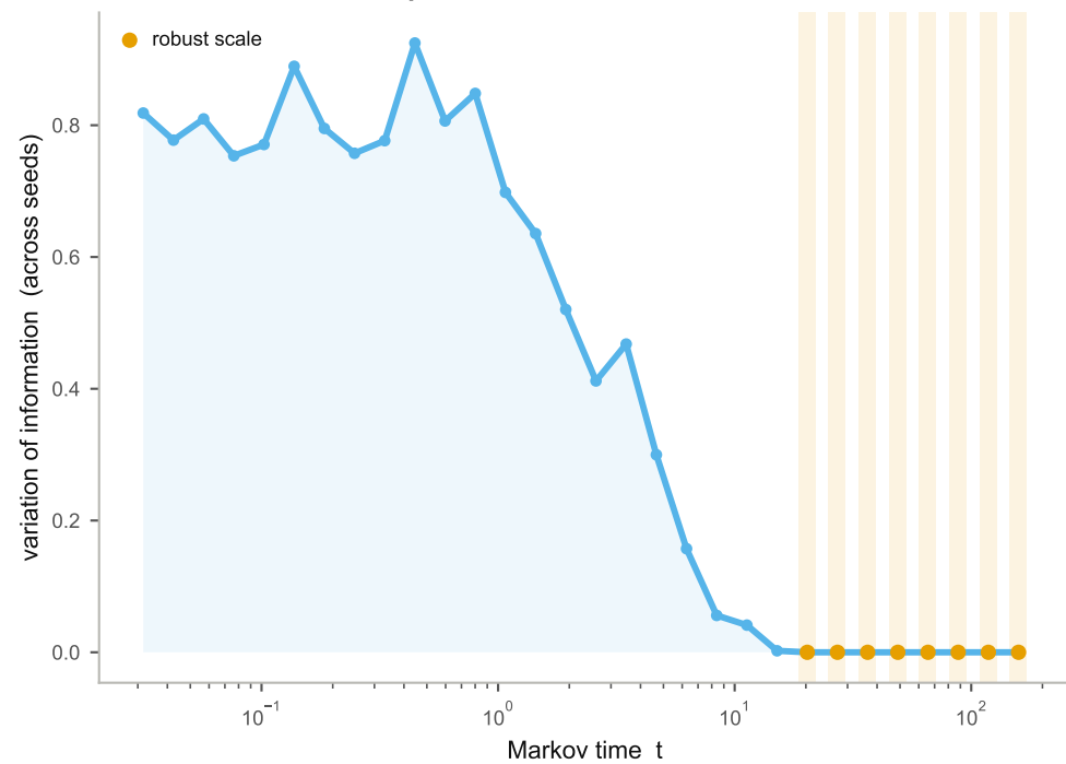
b Robust scales = low-VI plateaus
