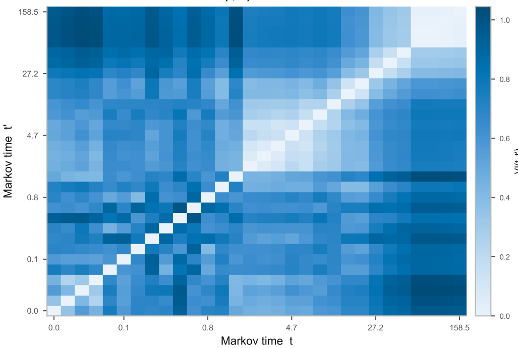
c Multiscale block structure VI(t, t')
