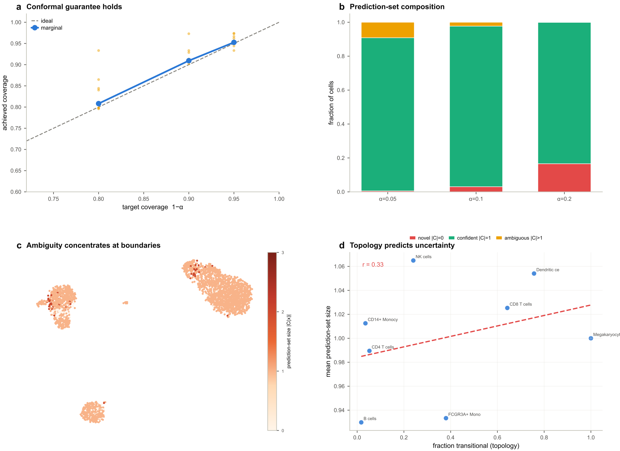
Figure 5 · Conformal prediction gives every cell a calibrated confidence set · pbmc3k
