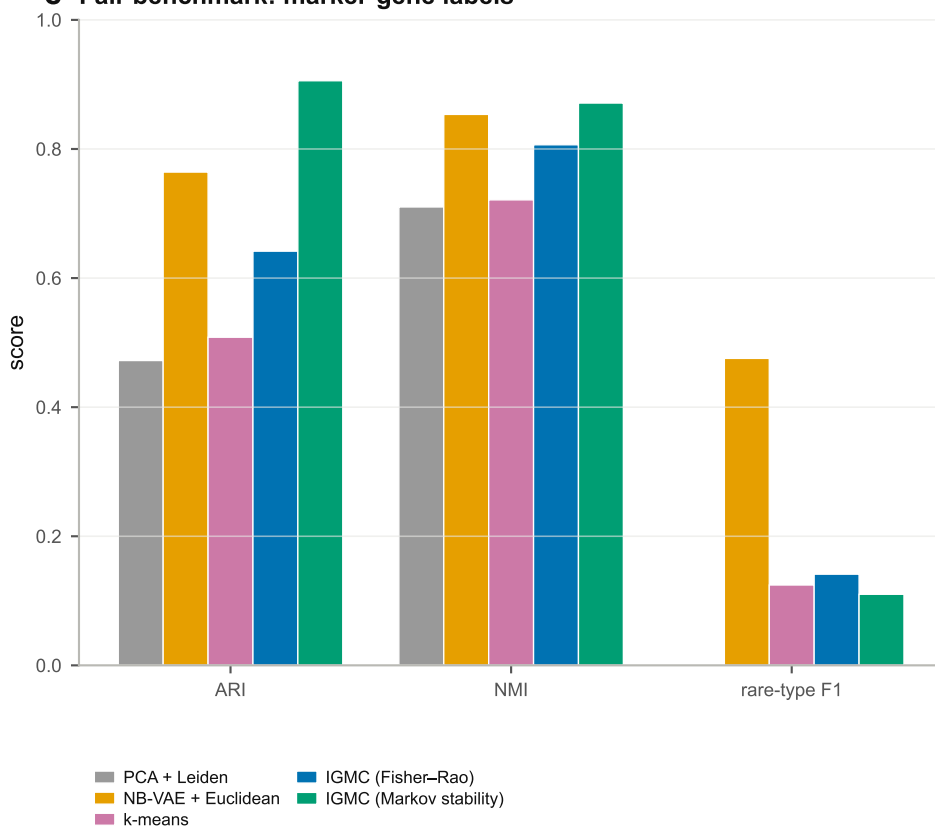
c Fair benchmark: marker-gene labels
