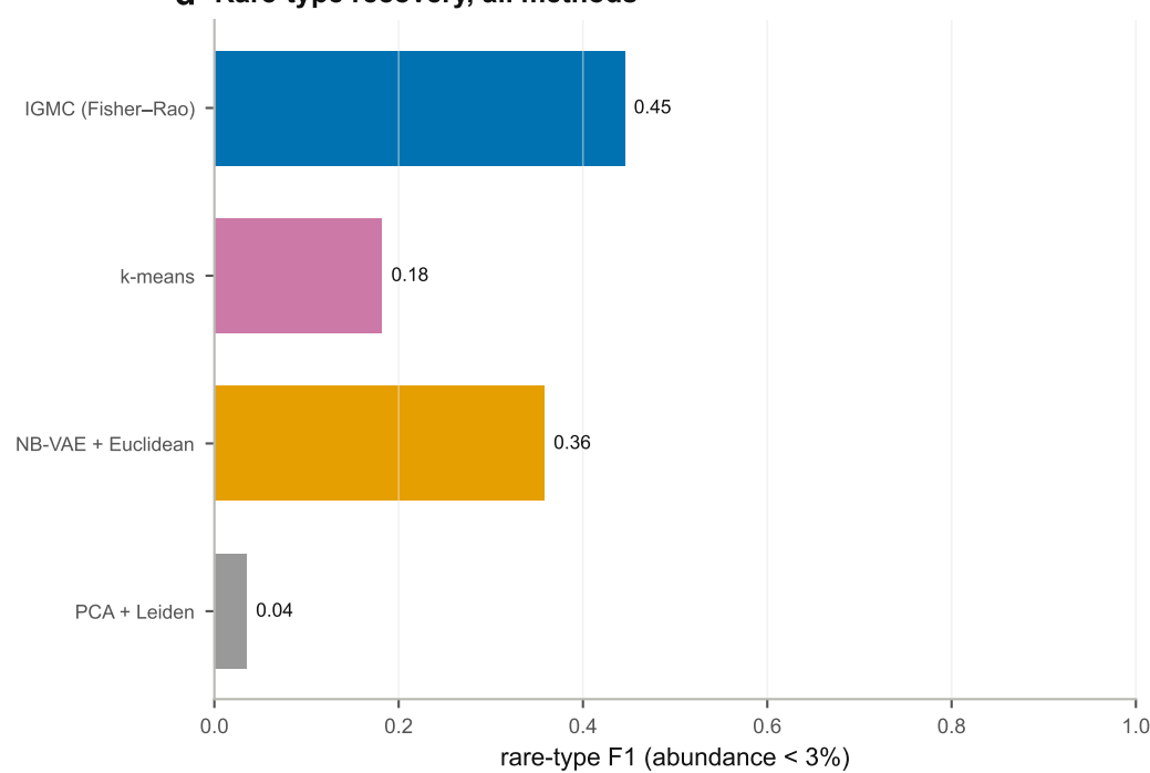
d Rare-type recovery, all methods
