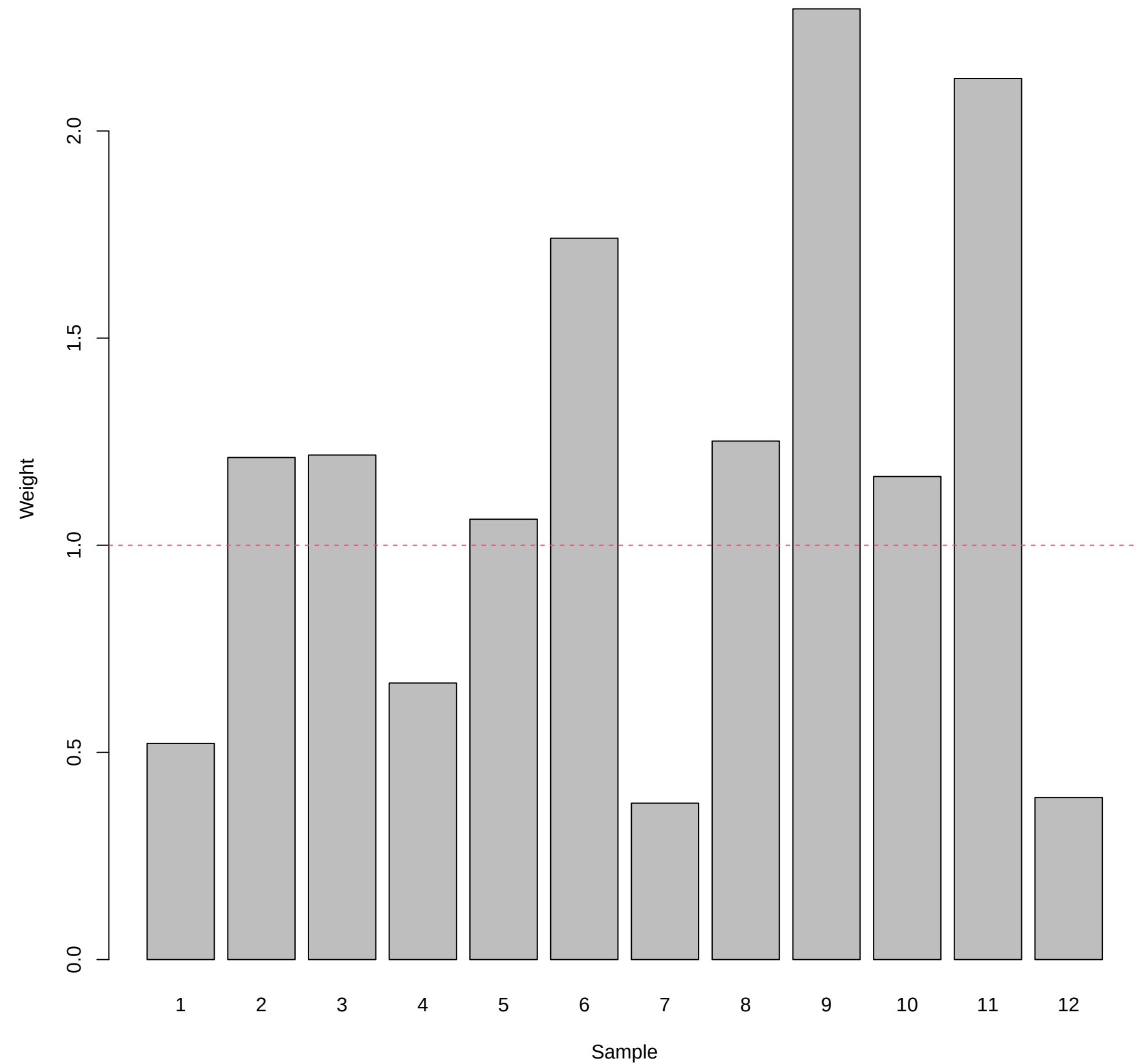
Sample-specific weights
