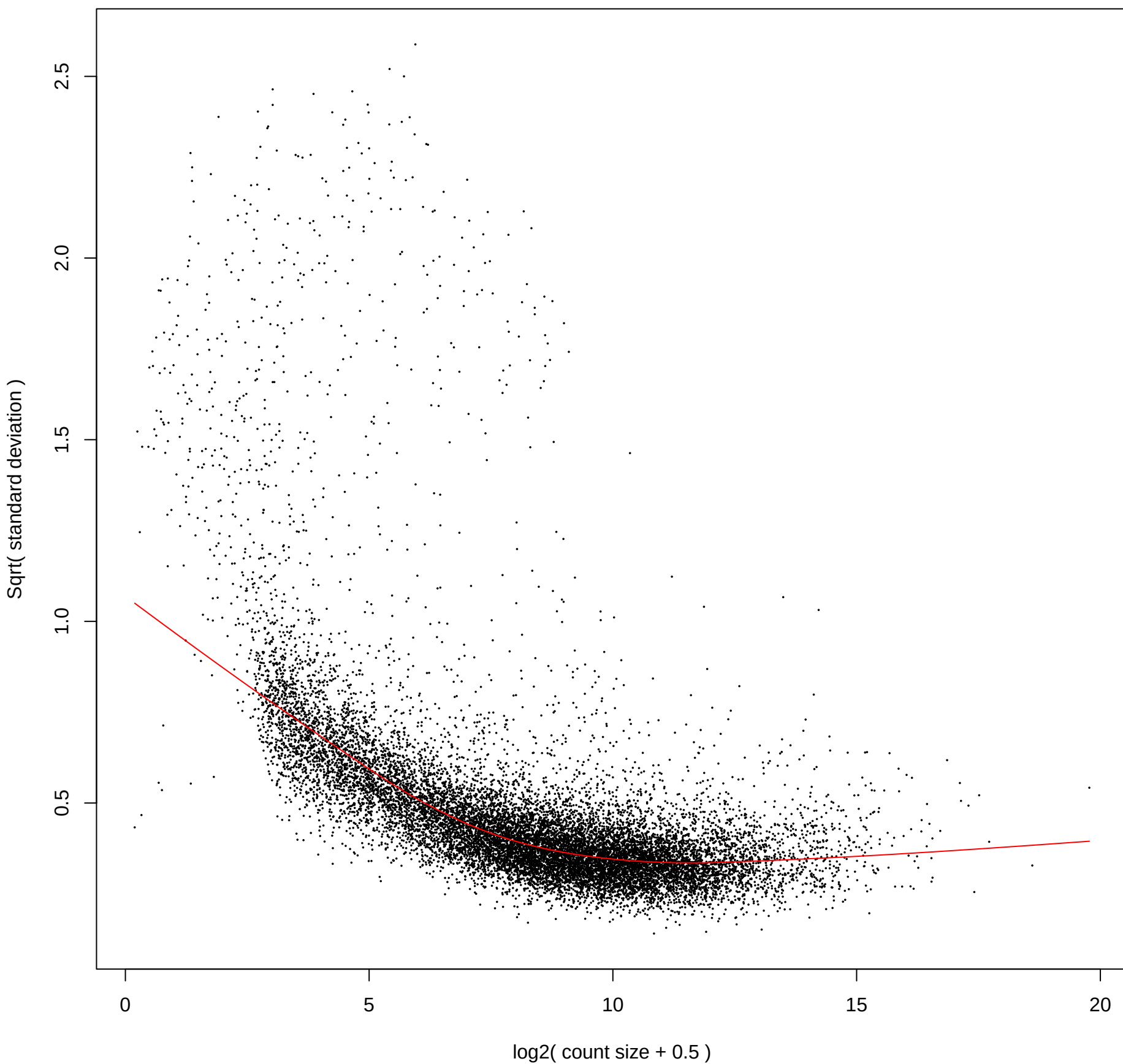
voom: Mean-variance trend
