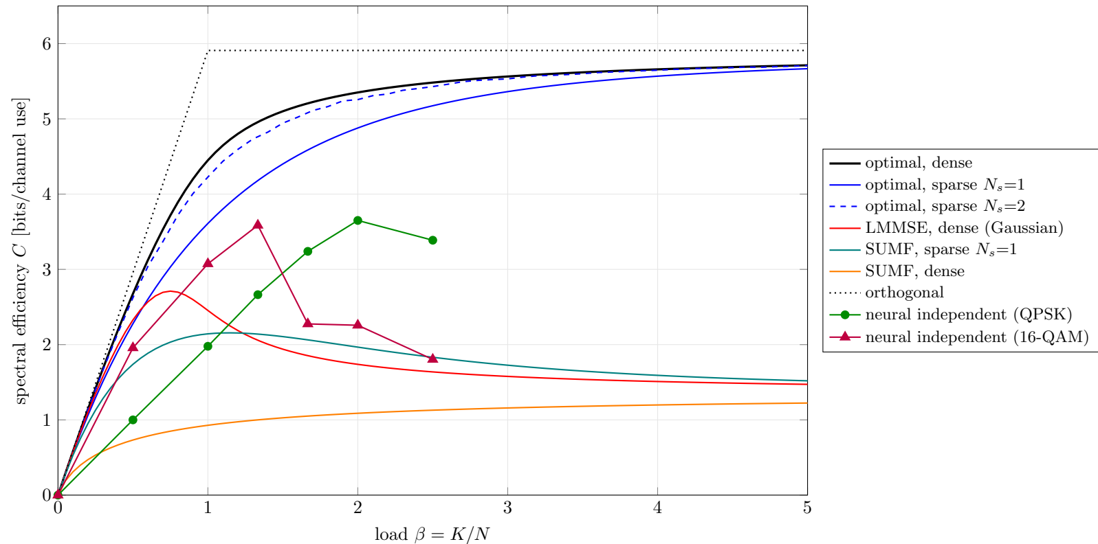
Large-system spectral efficiency, E_b/N_0 = 10 dB
