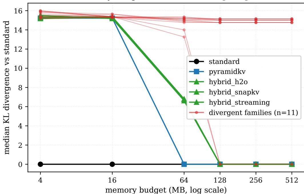
KL Pareto across memory budgets — Gemma 4 (50 prompts \times 16 strategies)
