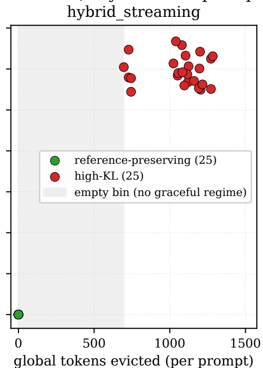
Gemma 4 global-eviction sensitivity at mb=64: empty band [1, 695] across 150 runs (3 hybrid × 50 prompts)
