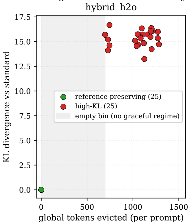
Gemma 4 global-eviction sensitivity at mb=64: empty band [1, 695] across 150 runs (3 hybrid × 50 prompts)
