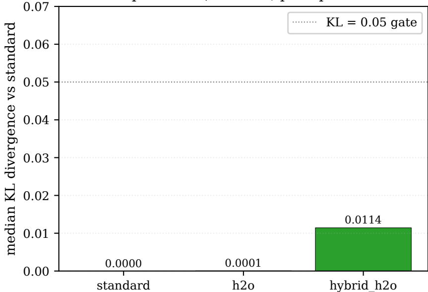
Gemma 2 scope check (mb=256, prompts \approx 7.7k tokens)
