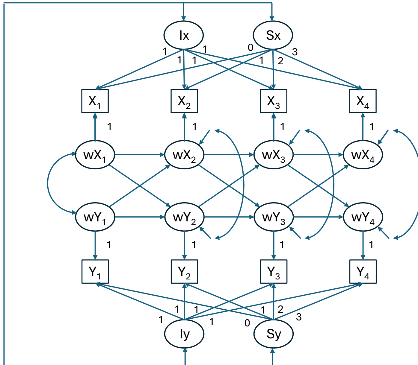
Latent Growth Curve Model With Structured Residuals (LGCM-SR)
