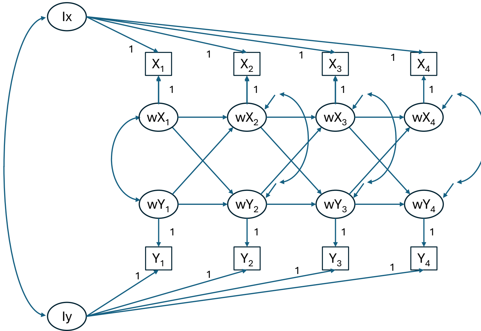
Random Intercept Cross-Lagged Panel Model (RI-CLPM)
