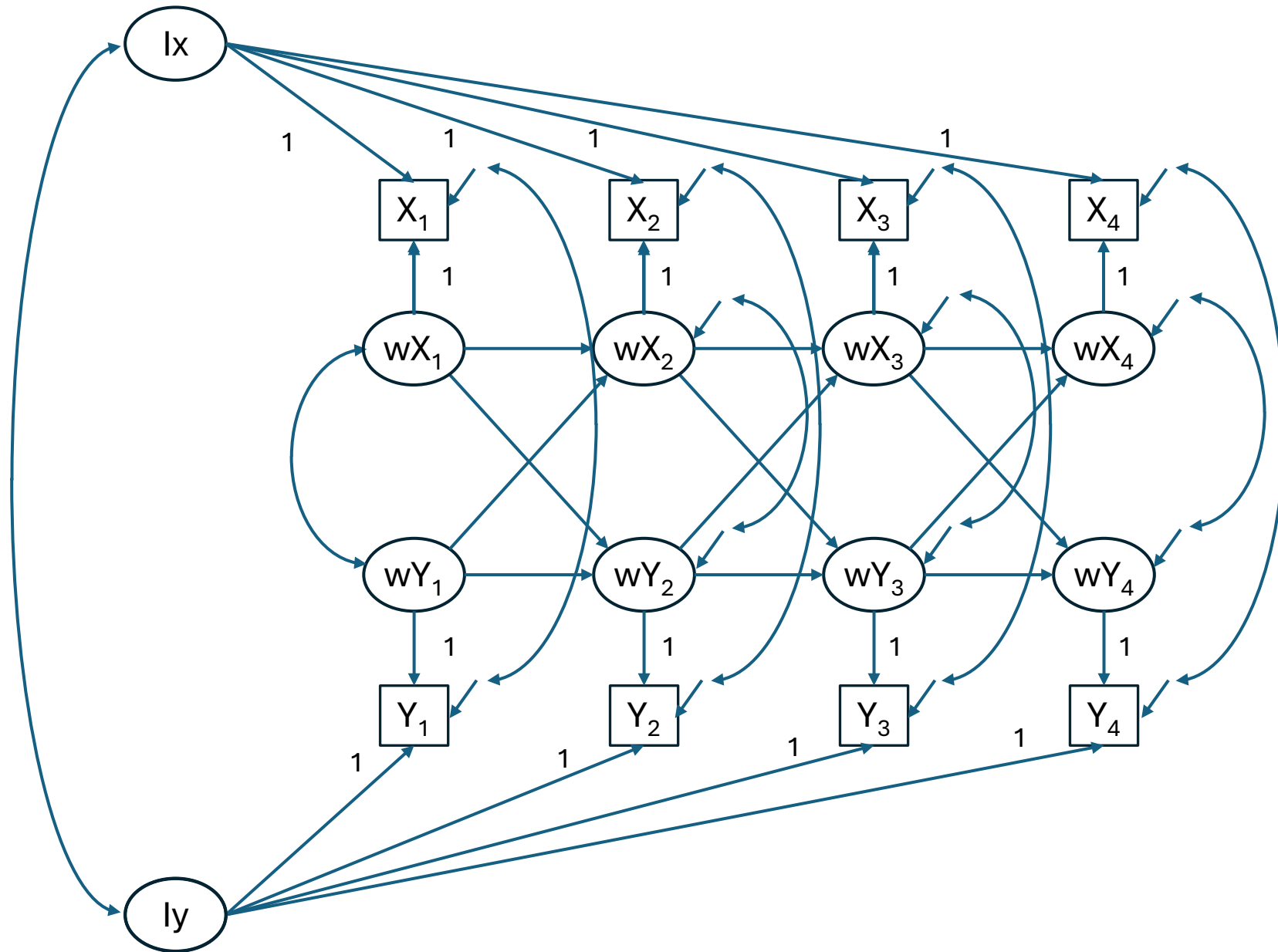
Stable Trait AutoRegressive Trait and State model (STARTS)
