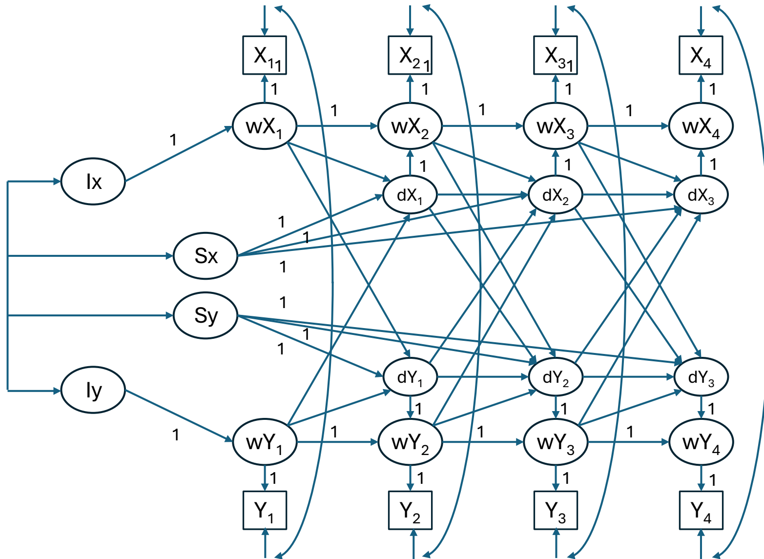
Latent Change Score Model with Changes-To-Changes Extension (LCS-CC)
