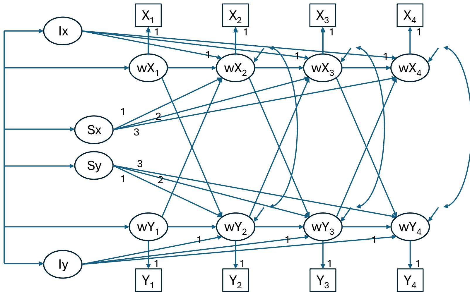
Autoregressive Latent Trajectory model (ALT)
