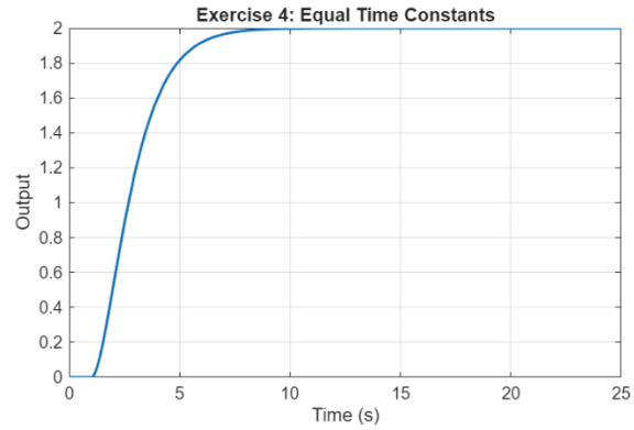
Figure 12. Equal time constant systems (series)
