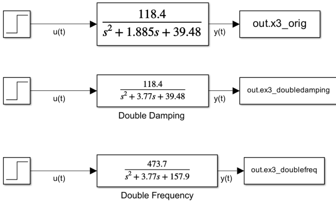
Figure 18. Exercise 3 Simulink
