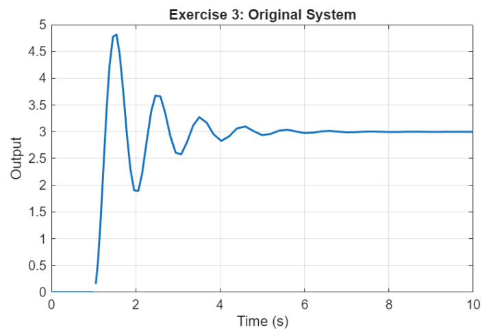
Figure 8. Original second-order system response
