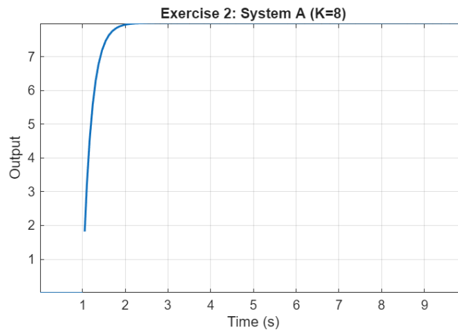
Figure 6. First-order system with high gain (System A)
