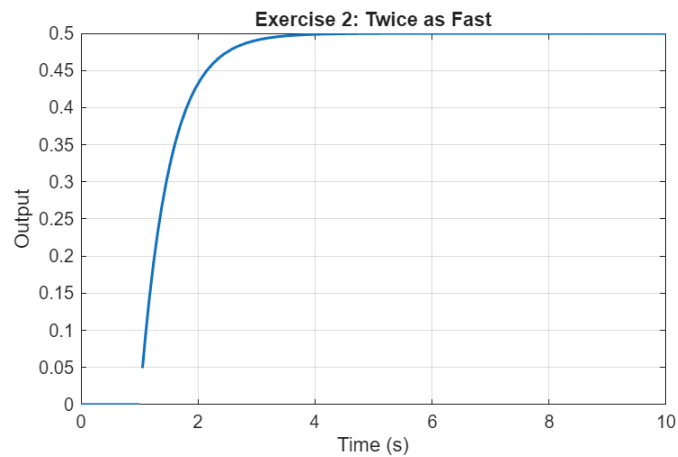
Figure 5. First-order system with reduced time constant
