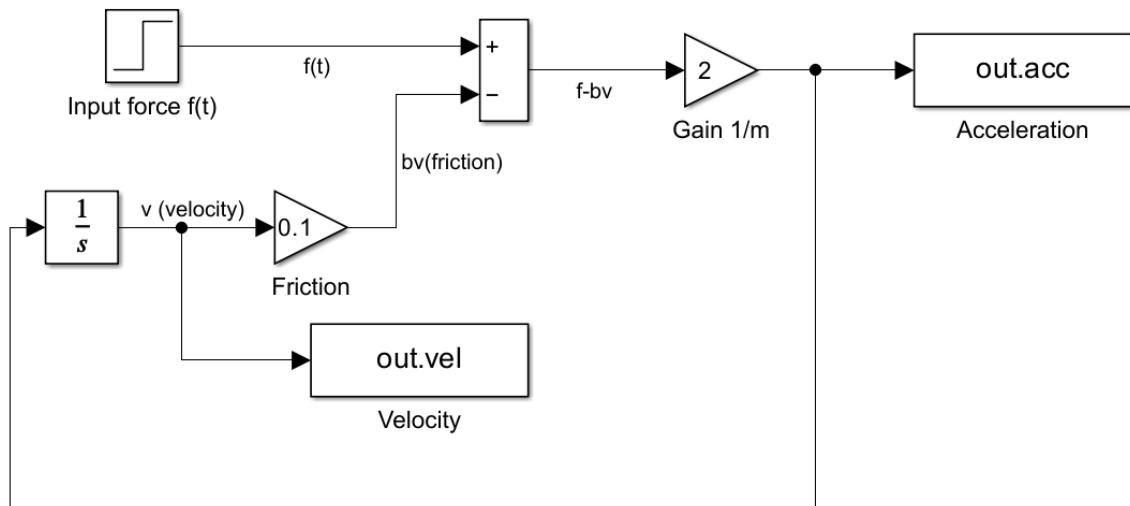
Figure 16. Exercise 1 Simulink
