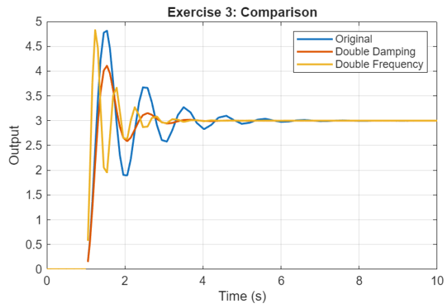
Figure 11. Comparison of second-order systems
