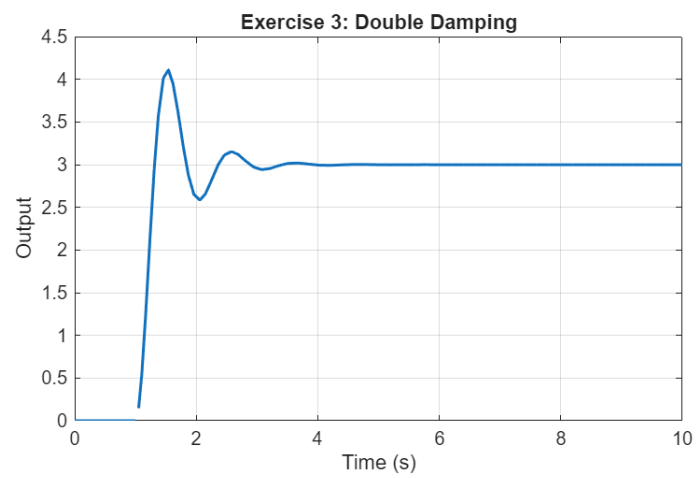
Figure 9. Second-order system with increased damping
