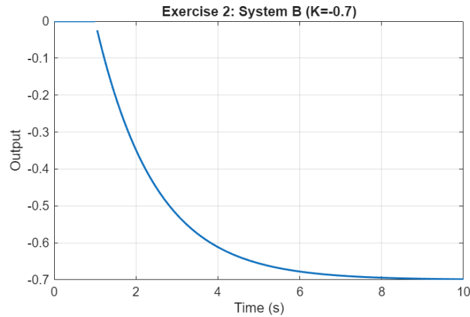
Figure 7. First-order system with negative gain (System B)
