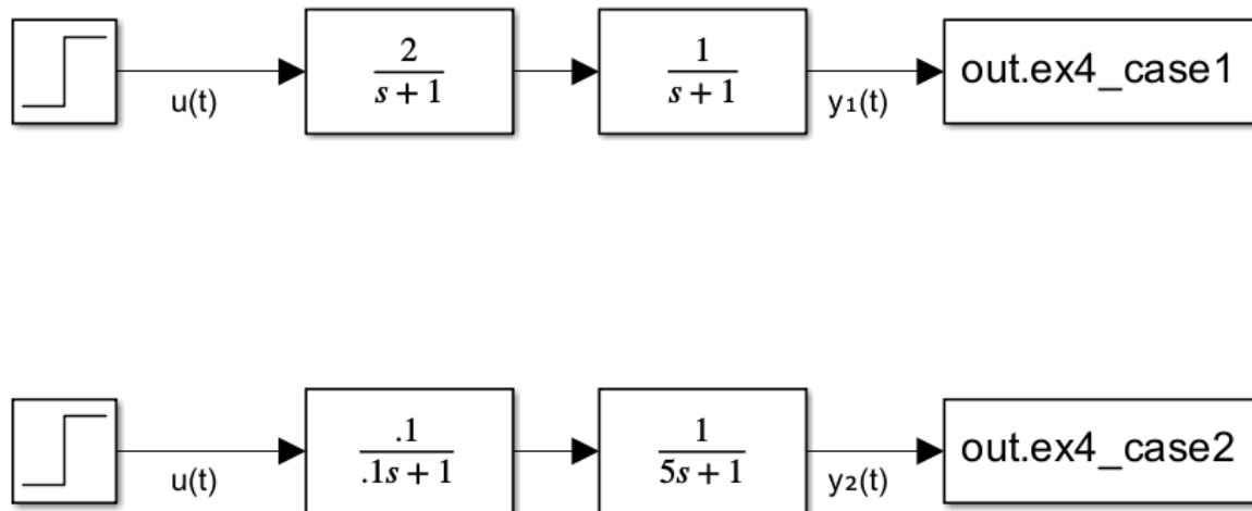
Figure 19. Exercise 4 Simulink
