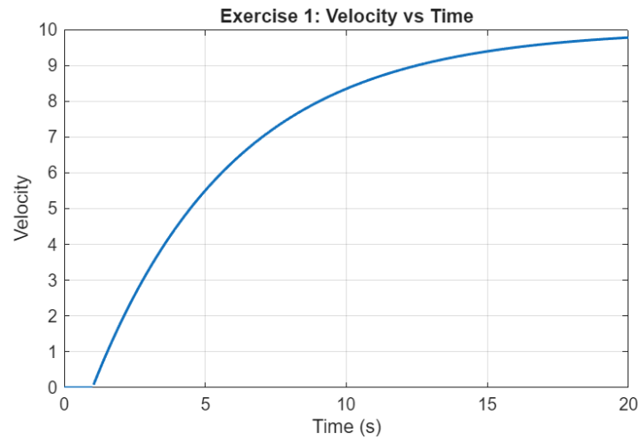
Figure 1. Velocity response of mass-damper system
