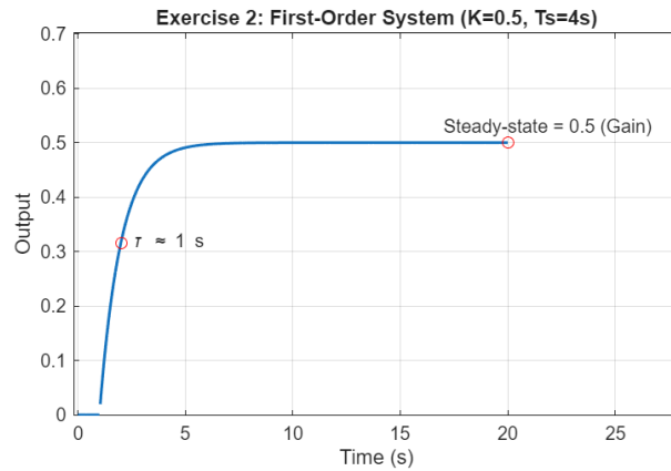
Figure 3. First-order system ( K=0.5 , T_s=4s )
