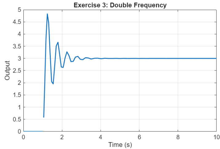
Figure 10. Second-order system with increased natural frequency
