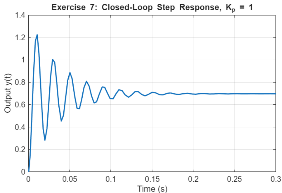
Figure 16. Closed-Loop Step Response with K_p=1
