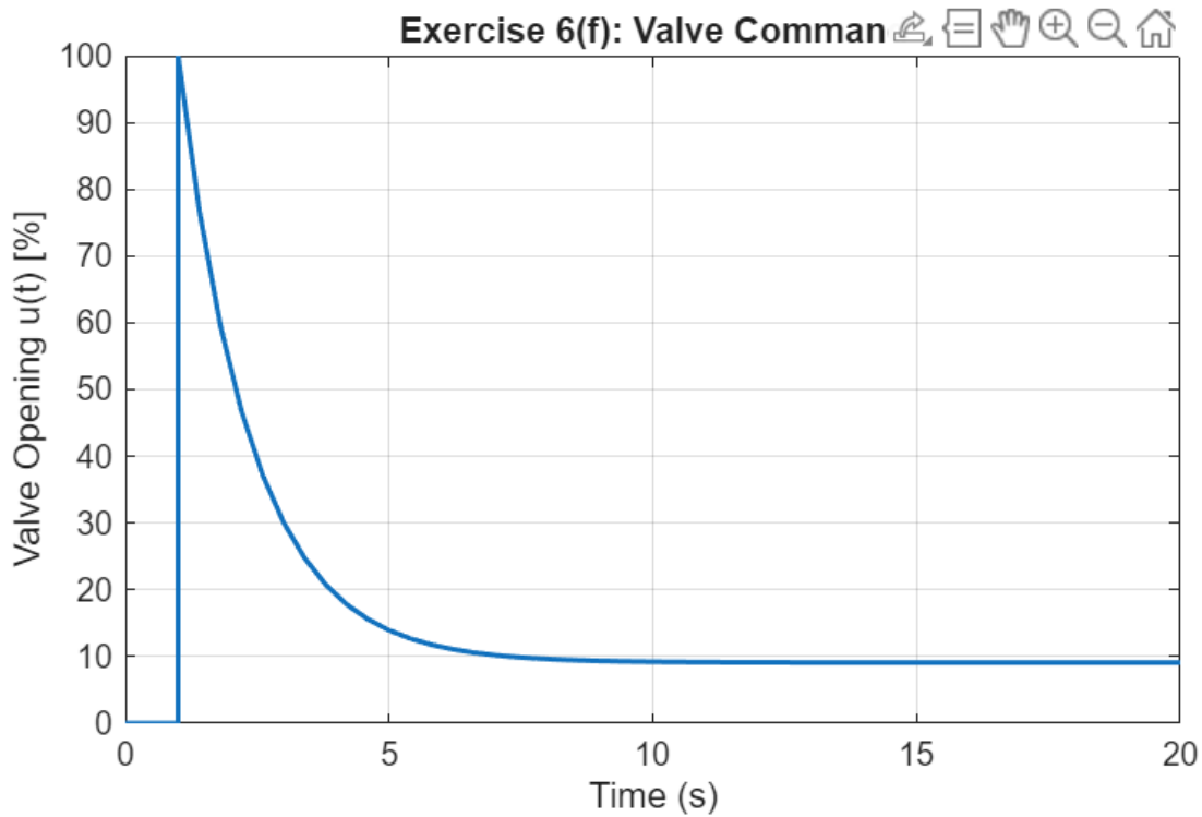
Figure 15. Final Valve Command
