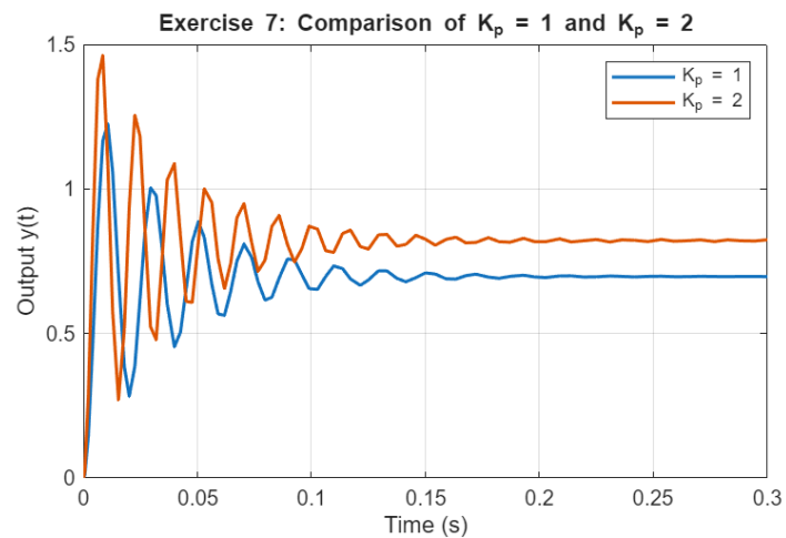
Figure 18. Comparison of Closed-Loop Responses for K_p=1 and K_p=2
