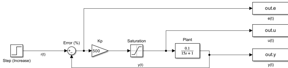
Figure 23. Model with Saturation
