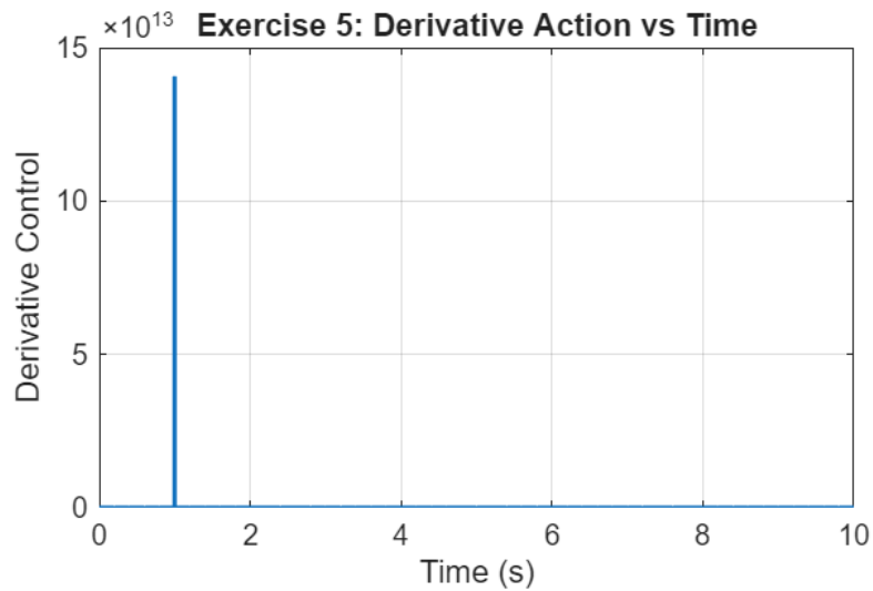
Figure 3. Derivative Control vs. Time
