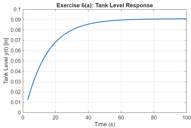
Figure 5. Tank Level Response
