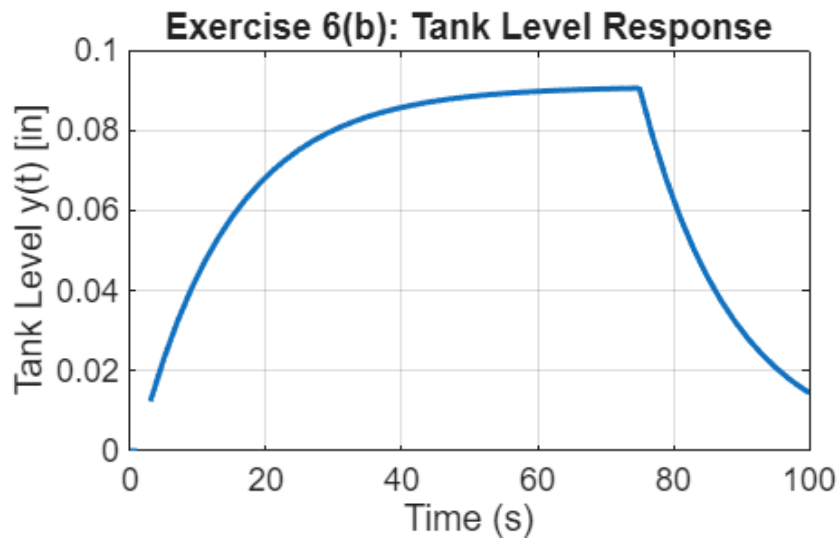
Figure 7. Tank Response with step increase and decrease
