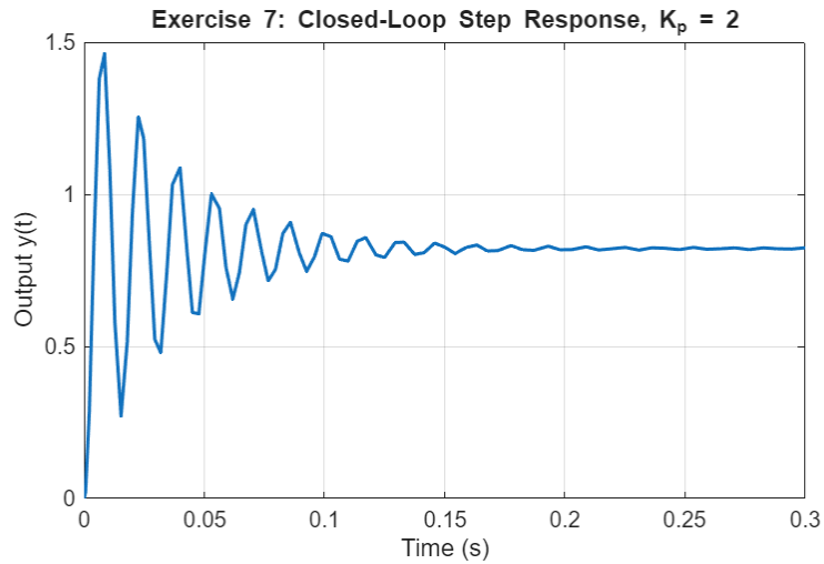
Figure 17. Closed Loop Response for K_p=2
