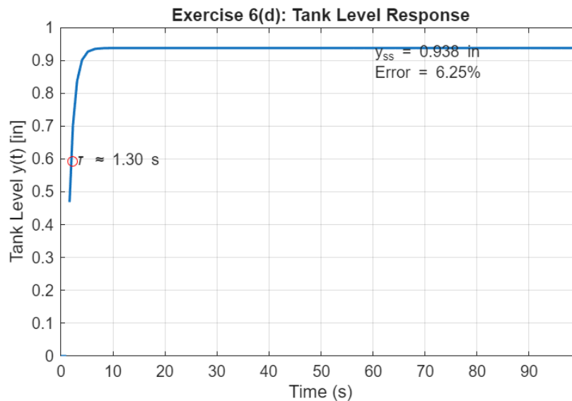
Figure 11. High Gain Response
