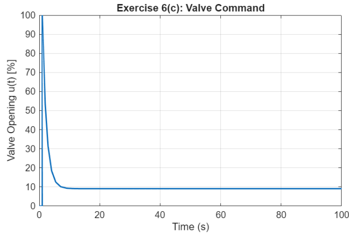
Figure 10. Gain Increase Valve Control
