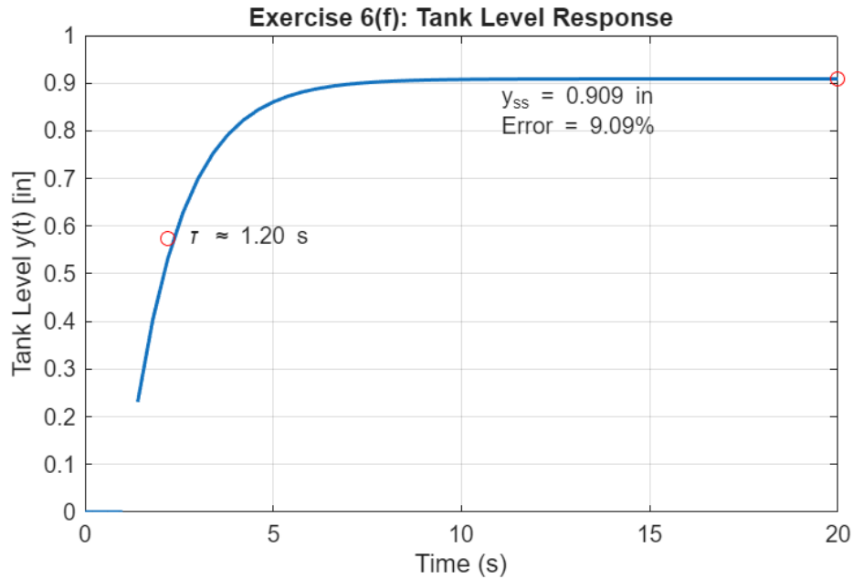
Figure 14. Final Response Without Saturation
