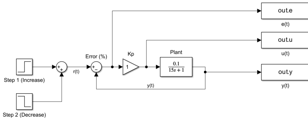
Figure 22. Increase and Decrease Step Input Model
