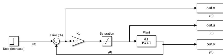
Figure 24. Redesigned Controller Model
