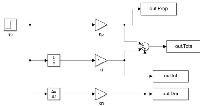
Figure 20. Exercise 5 Simulink Model
