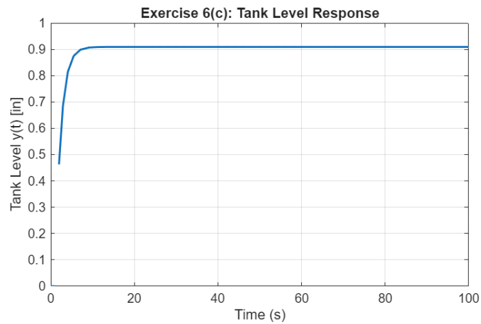
Figure 9. Improved Response with Increased Gain
