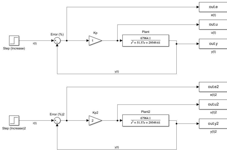
Figure 25. Second-Order Closed-Loop Model
