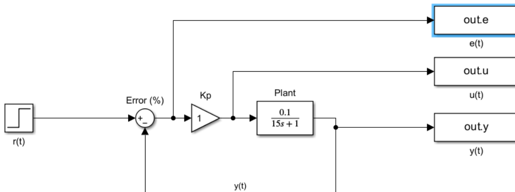
Figure 20. Exercise 5 Simulink Model
