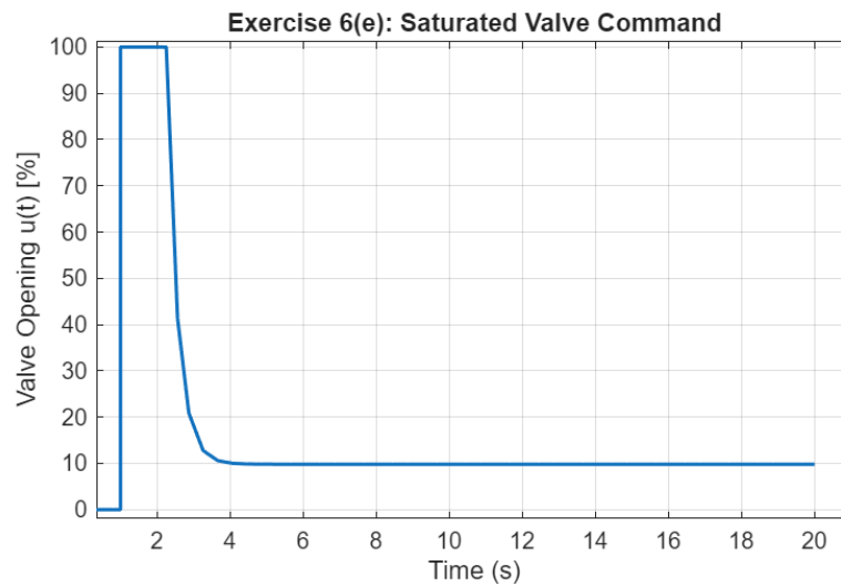
Figure 13. Valve Command with Saturation
