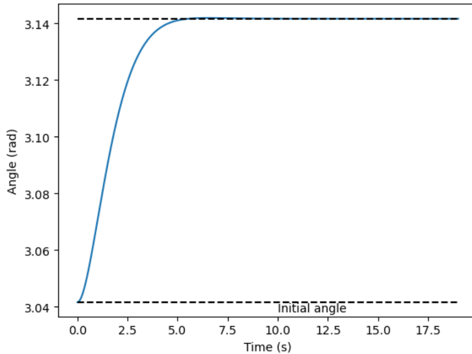
Figure 1. Angle( \theta ) Vs. Time (s) Model Response
