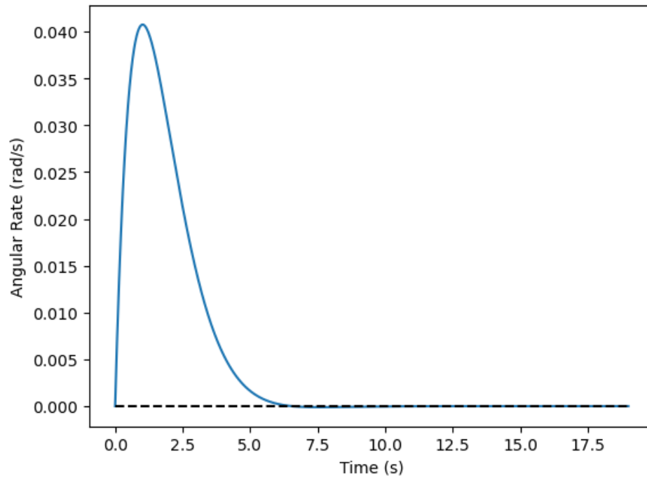
Figure 2. Angular Velocity( \dot{\theta} ) Vs. Time (s) Model Response
