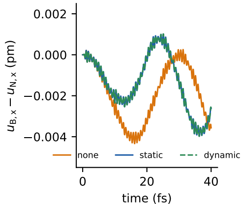
HSEX, laser 8 eV
