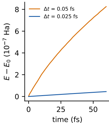
HSEX, RK4 energy drift
