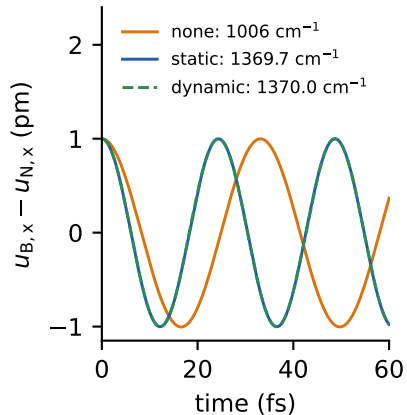
HSEX, no laser
