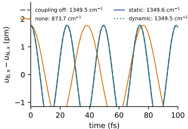
real hBN, IPA, no laser
