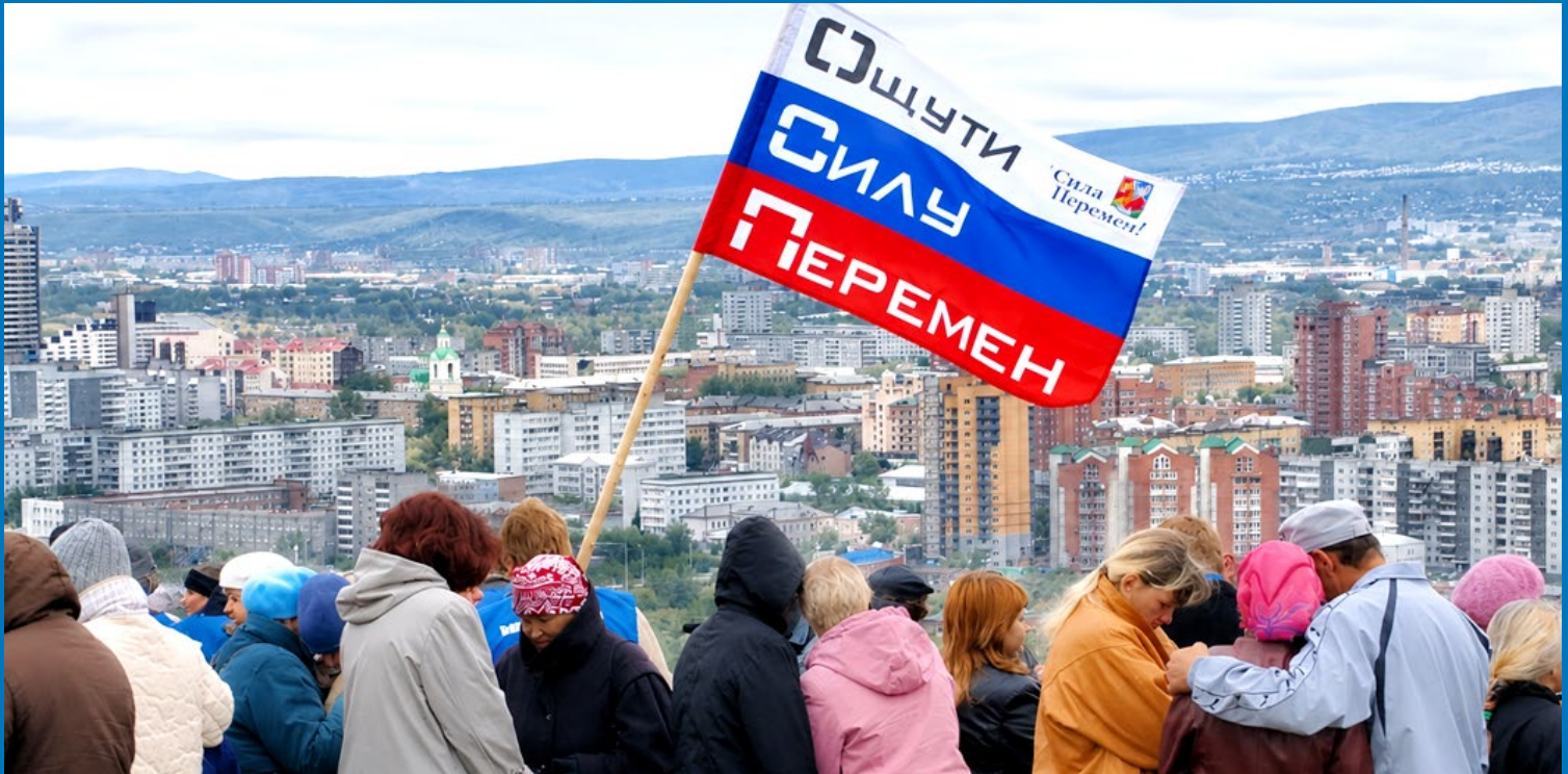
2007 Krasnoyarsk, Eastern Siberia
