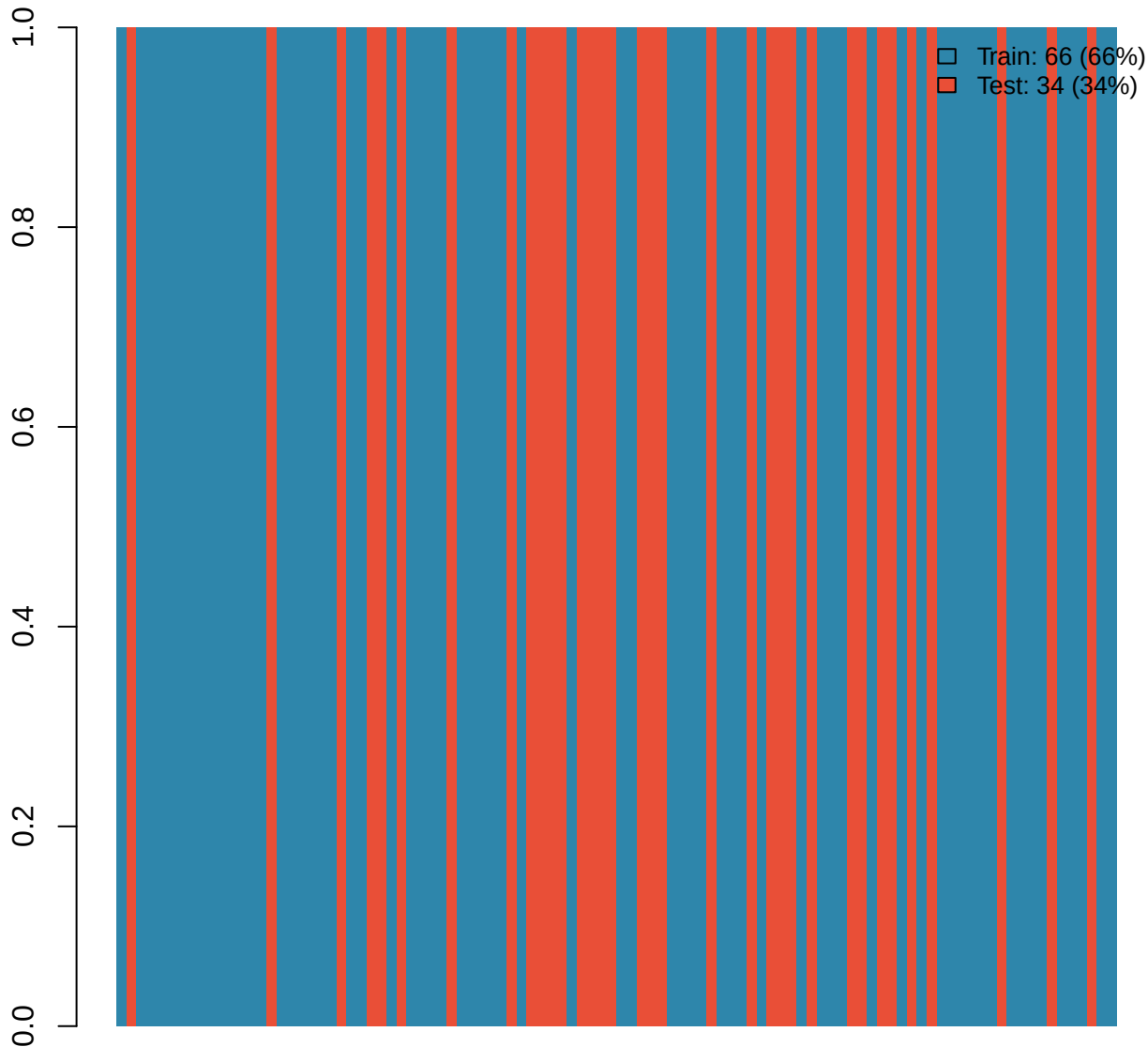
Fold 1 Split
