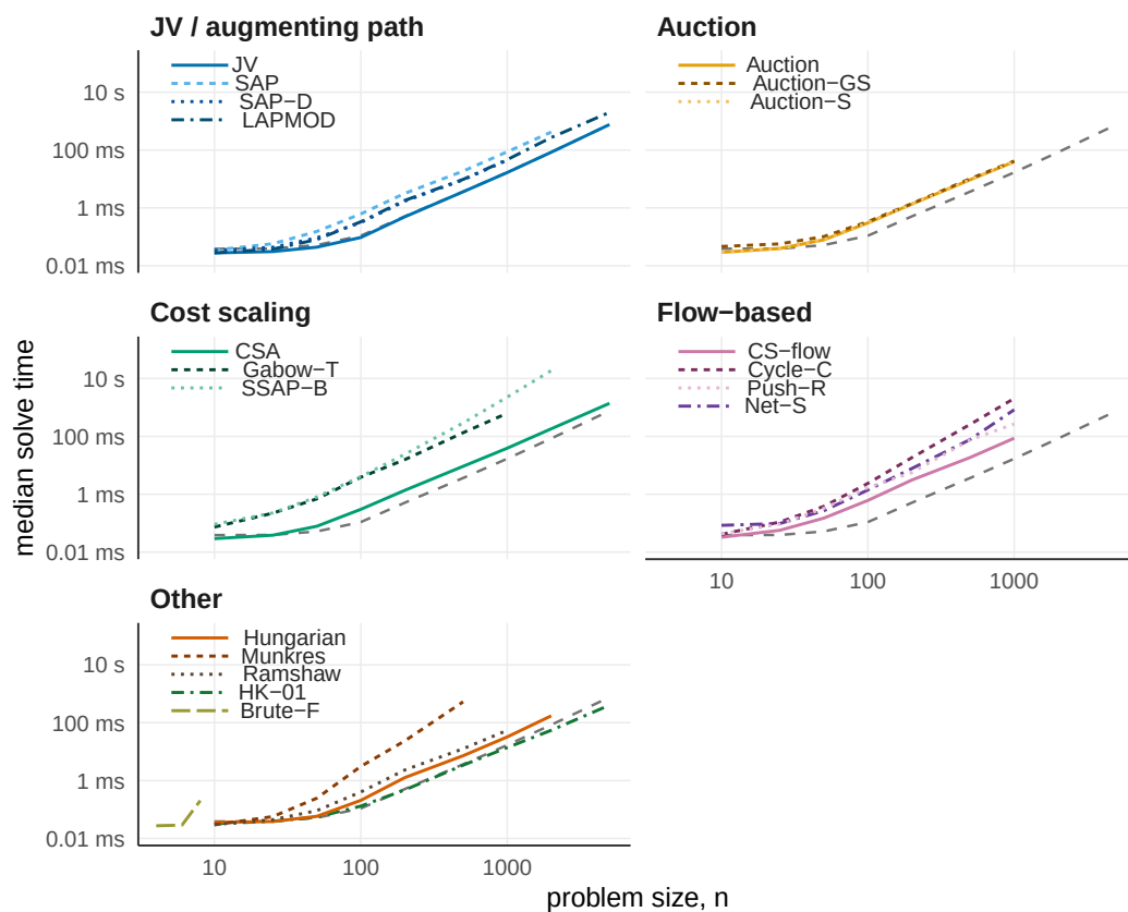
Figure 1: Median wall-clock solve time against problem size for the nineteen assignment solvers in couplr, grouped by algorithm family on shared log-log axes. Seventeen solvers are timed on square integer cost matrices with entries drawn uniformly from 1 to 10,000. The two special-purpose solvers in the Other panel run on their own inputs and are not comparable to the rest: HK-01 is timed on binary cost matrices, and Brute-F only up to n = 8 . The dashed grey line repeated in every panel is the automatic dispatcher on the uniform integer costs. Medians of five replicates on a single core of an Apple M4 Pro. Cubic-time and general flow solvers are capped at smaller sizes, which is why their lines end early.
