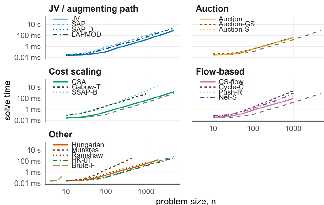
Figure 1: Wall-clock solve time, the fastest of five interleaved repetitions, against problem size for the nineteen assignment solvers in couplr, grouped by algorithm family on shared log-log axes. The two special-purpose solvers in the Other panel run on their own inputs and are not comparable to the rest: HK-01 is timed on binary cost matrices, and Brute-F only up to n = 8 . The dashed grey line repeated in every panel is the automatic dispatcher on the uniform integer costs.
