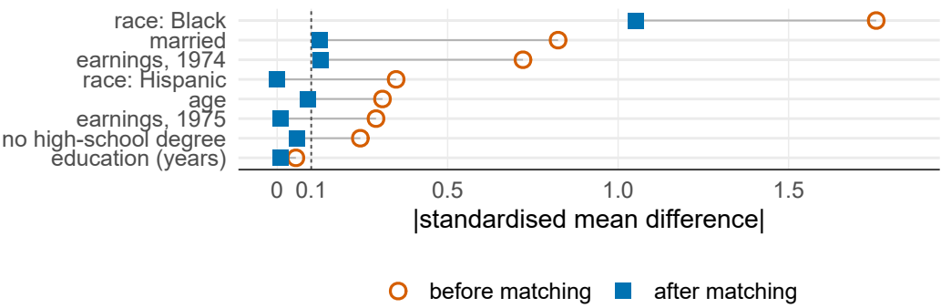
Figure 2: Absolute standardised mean differences on the eight LaLonde NSW covariates, before and after one-to-one optimal Mahalanobis matching with pooled within-group covariance. couplr, MatchIt and optmatch agree to three decimal places after matching, so a single matched point is shown per covariate. The dashed line marks the conventional 0.1 threshold. The indicator for Black respondents starts far outside the plotted range at 1.757 and remains at 1.053 after matching, a residual imbalance that no one-to-one matcher can resolve on this data.
