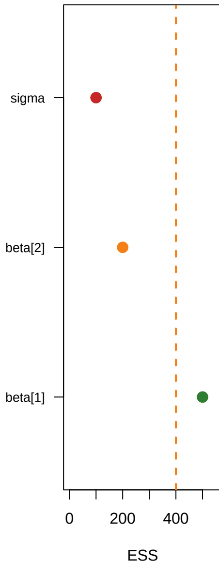
Effective Sample Size (bu
