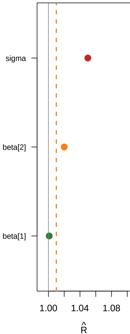
Rhat Convergence Diagno
