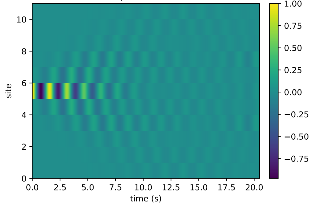
interpolated Cs.imag
