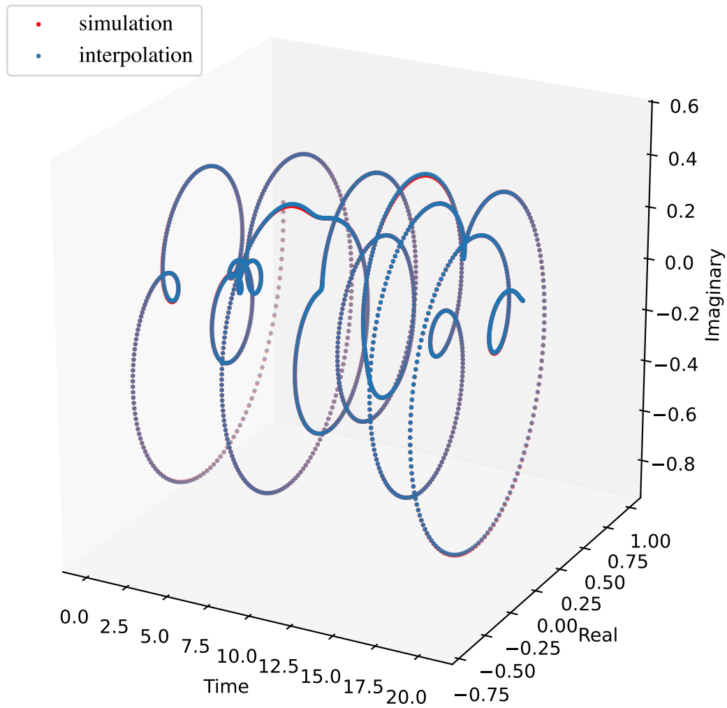
Interpolated vs Theoretical corr. in 3D
