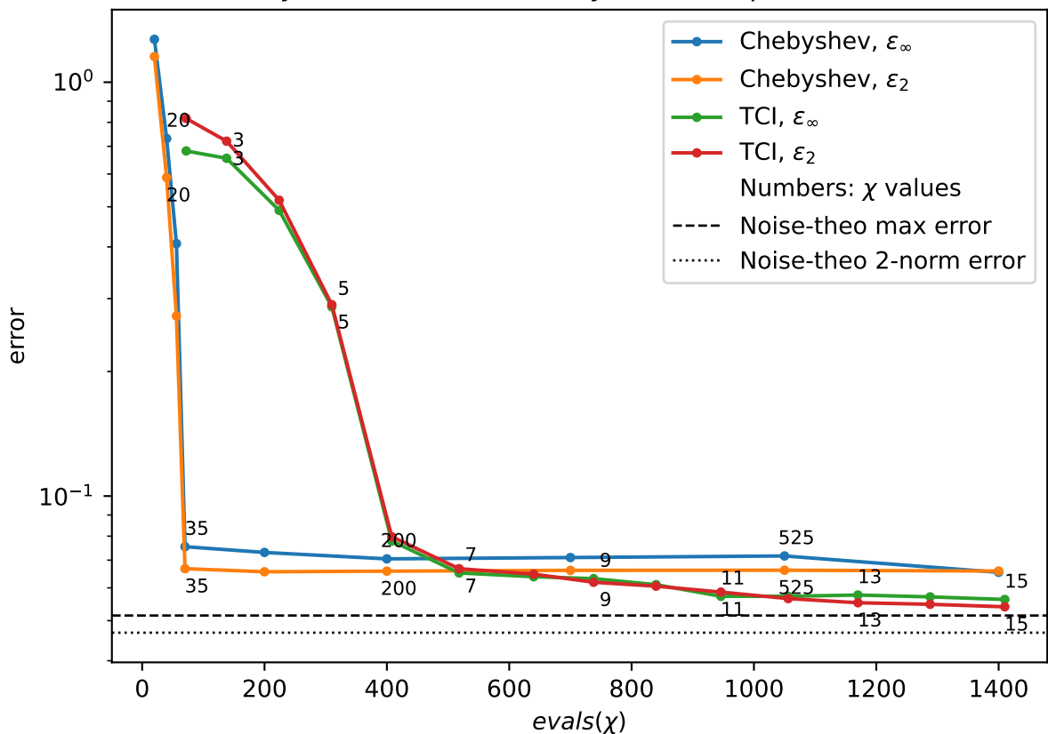
Error between noisy correlator and Chebyshev interpolation vs # of evalua
