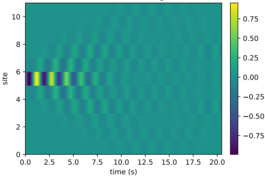
theoretical Cs.imag
