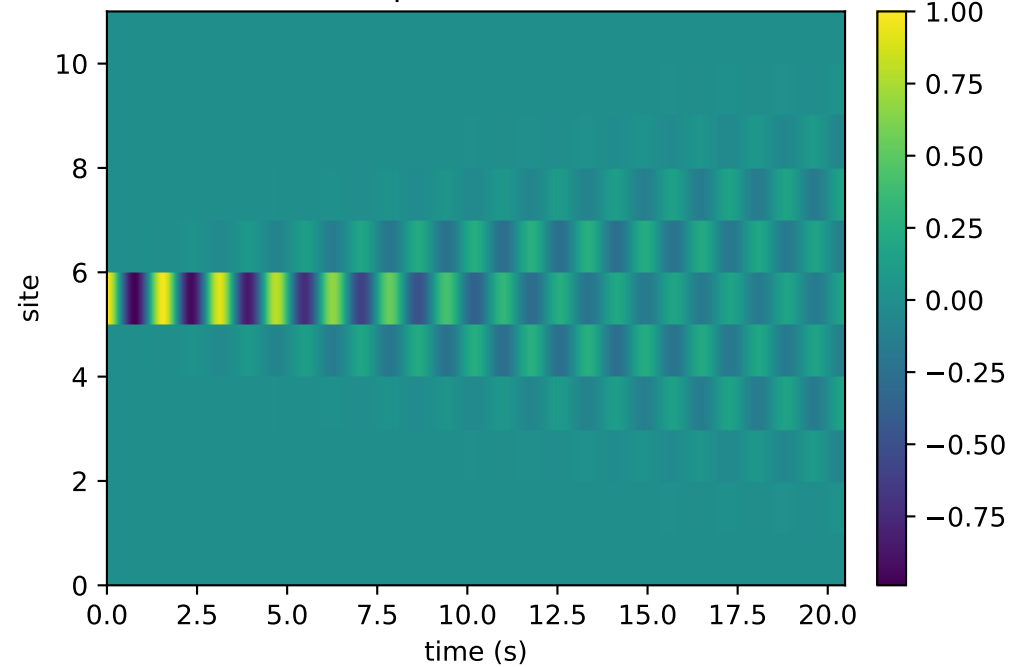
interpolated Cs.imag
