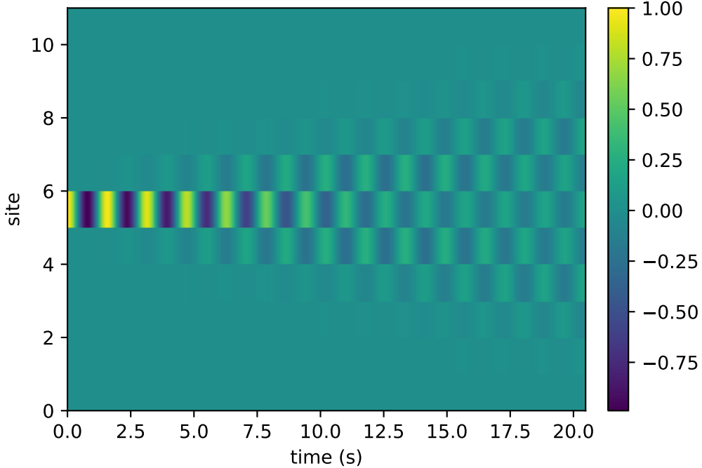
theoretical Cs.imag
