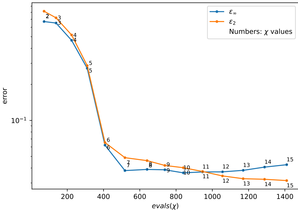
Error vs # of evaluations
