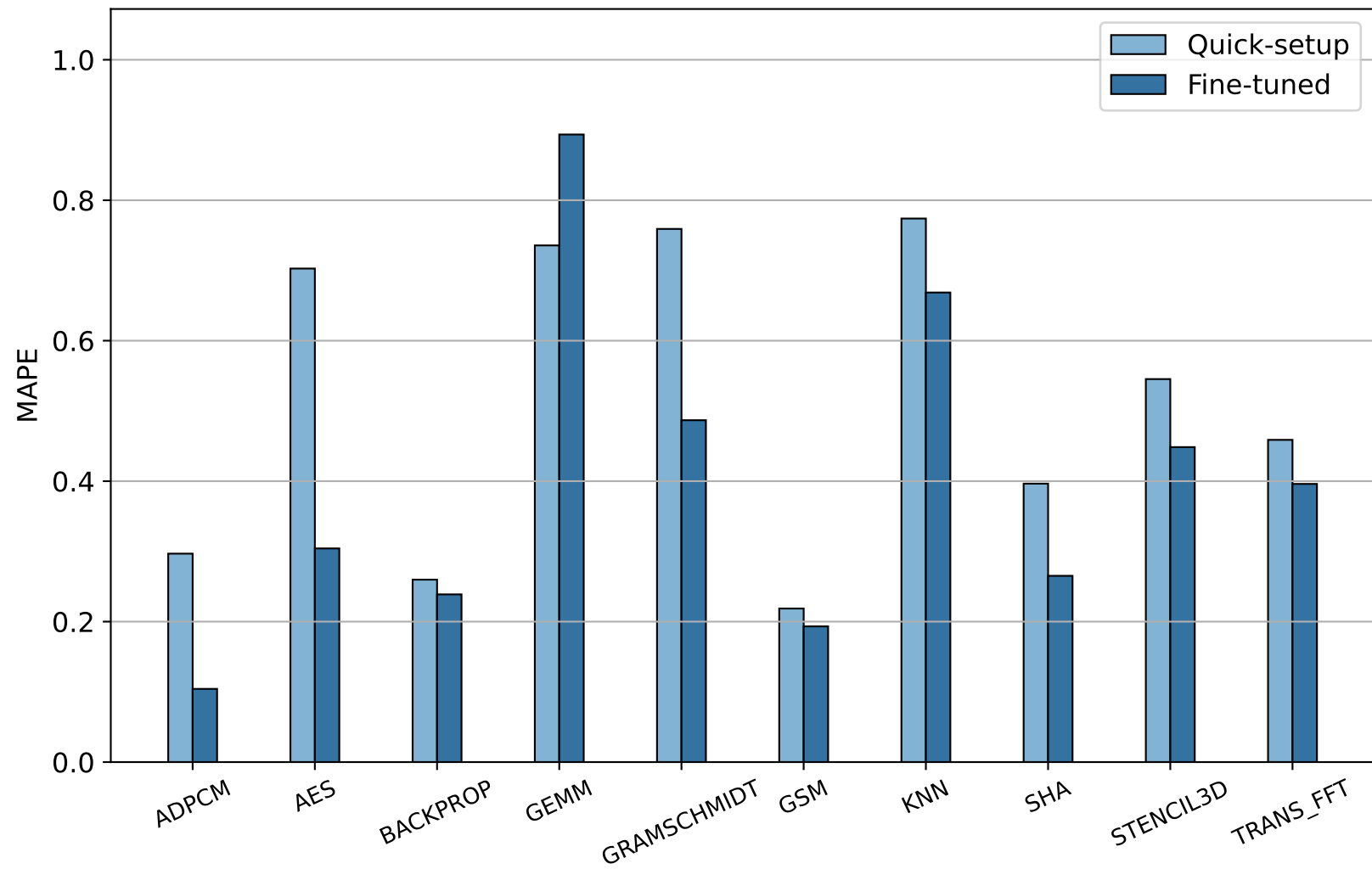
Per-Benchmark Model Performance
