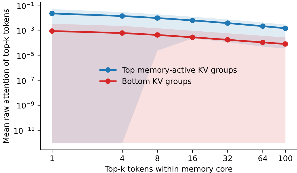
Memory-core top-k attention
