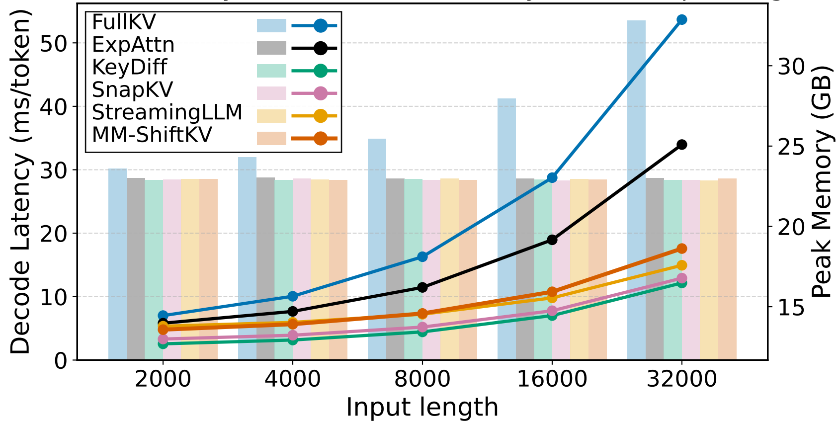
Decode Latency (bar) and Peak Memory (line) vs Input length
