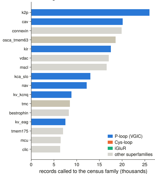
B The largest families
