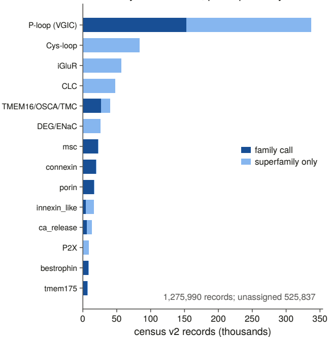
A Called by domain rules, per superfamily
