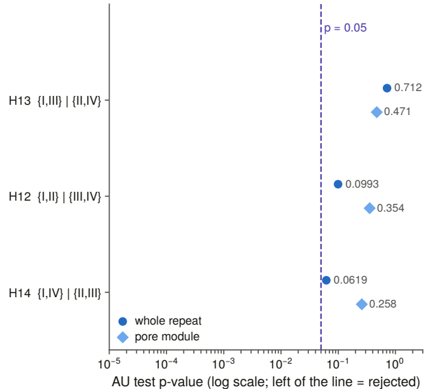
B Which repeats pair: AU test
