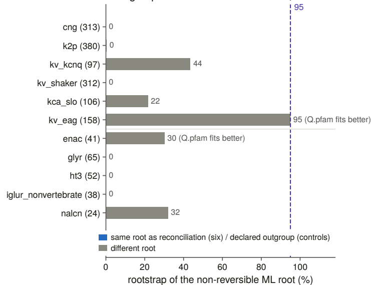
C Outgroup-free roots: S7d's six above, controls below
