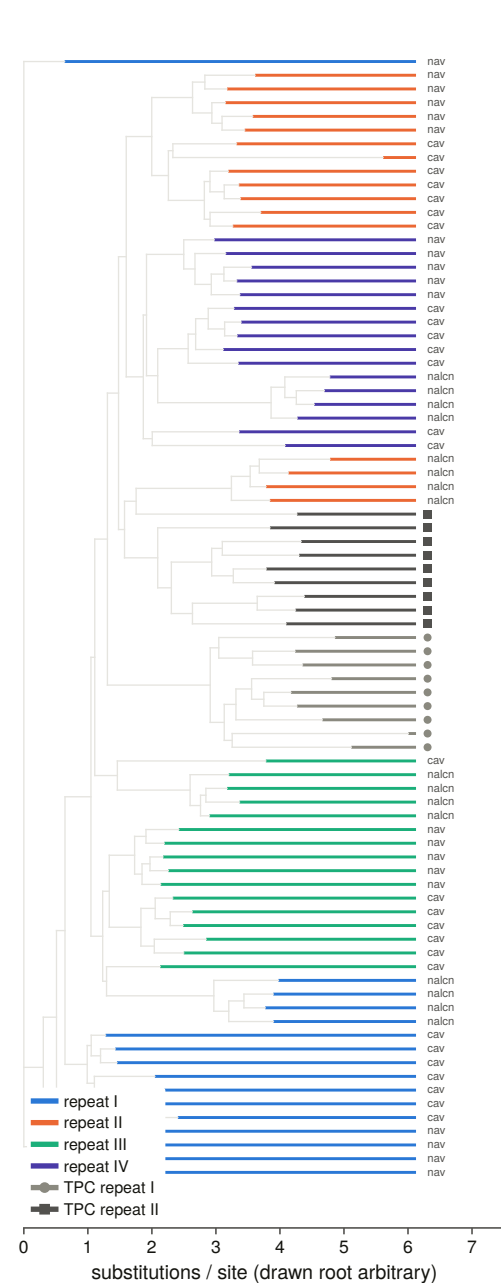
A Whole S1–S6 repeats, 82 tips (unrooted)
