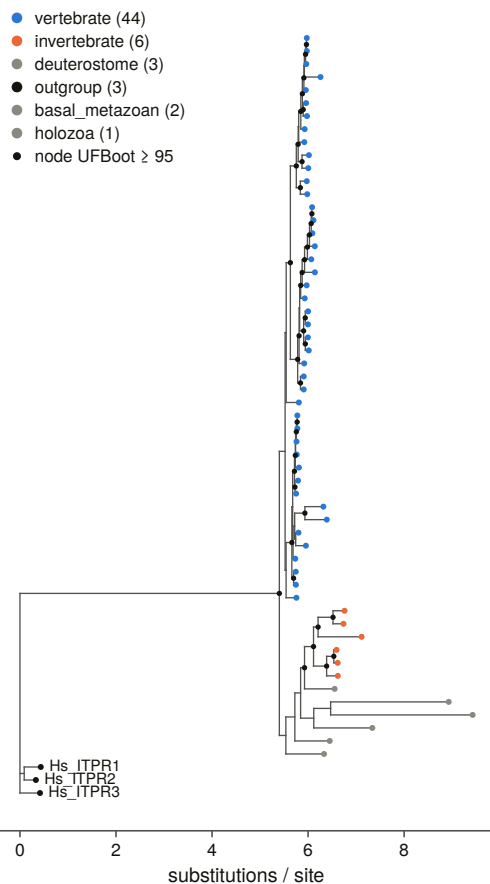
D Ryanodine receptors, rooted on ITPR
