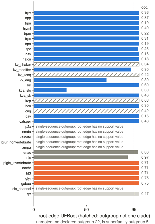
C Roots from the catalogue's outgroups
