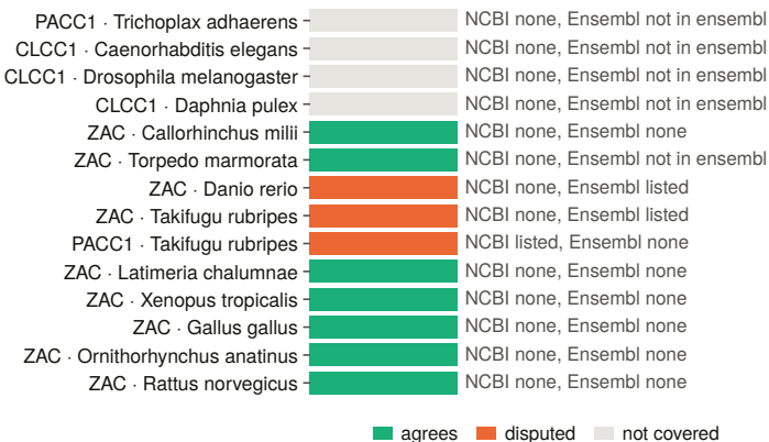
C S5 absences against two ortholog databases
