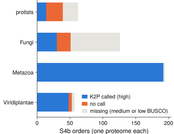
D K2P calls by kingdom
