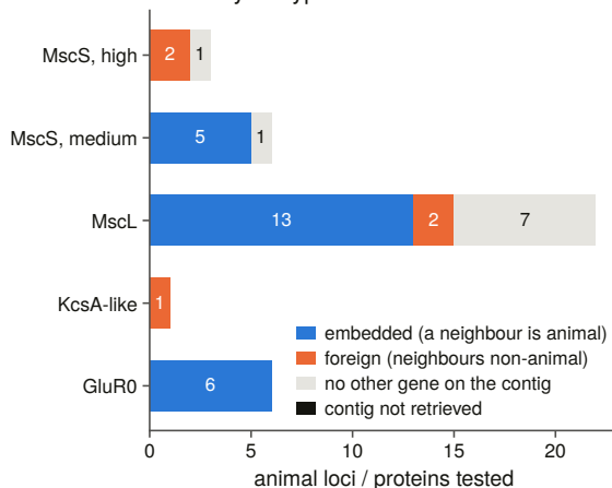
A Prokaryote-type channels in animals: what is on their contig
