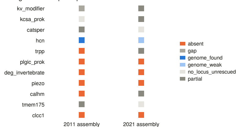
B Daphnia pulex: S5 verdicts on two assemblies
