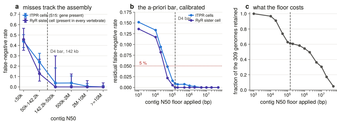
Extended Data Fig. 2 | The vertebrate genomic sweep and its contiguity confounder. (a) What the sweep found for each paralogue and for the ryanodine receptor positive control across all 309 genomes. (b) Recovery against assembly contiguity, binned on the contiguity bar rather than across it, and the same comparison as a two-bar contrast either side of it: 98–99 % of cells are found above the bar against 57–70 % below it, and below the bar the ordering is ITPR3 > ITPR1 > ITPR2 , which is the order of their gene spans. (c) Loci found per genome for each paralogue, with the ryanodine receptors beside them: the ITPR1 second copy in the ray-finned fish is the only substantial multi-copy signal in the family, against two to six copies for the control, whose three genes the sweep most often recovers as two or three loci.
