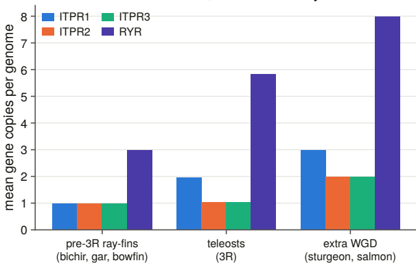
a 3R doubled ITPR1 alone, and all three RyRs
