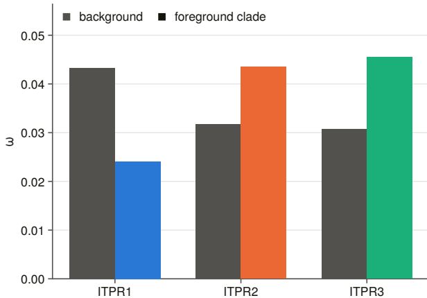
a Two-ratio models test each clade against the rest
