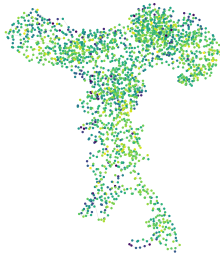
b ITPR2 (9YKK) resolves 2,168 residues
