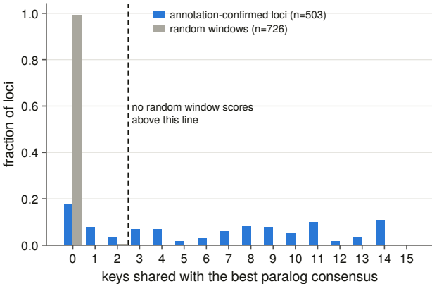
a Confirmed loci overlap the consensus far more than random windows do
