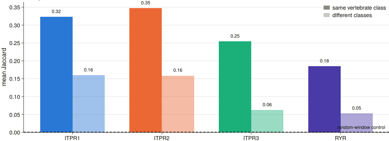
Neighbourhood conservation is lower across vertebrate classes than within them
