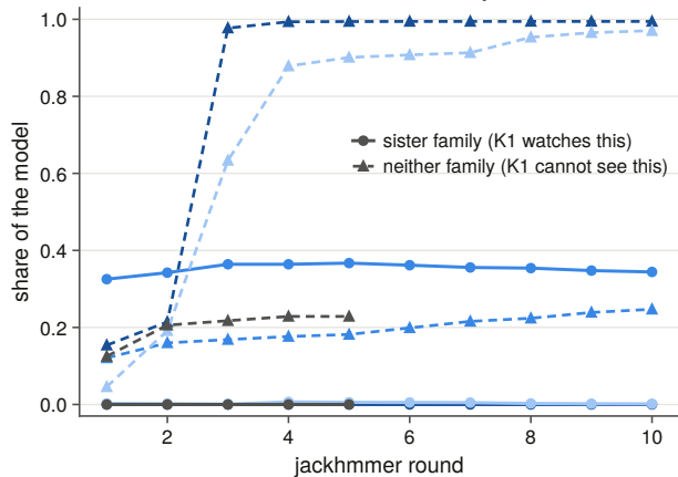
b Drift shows in the sister and off-family shares
