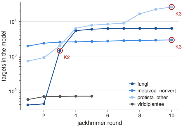
a Each run converges, or D10 kills it
