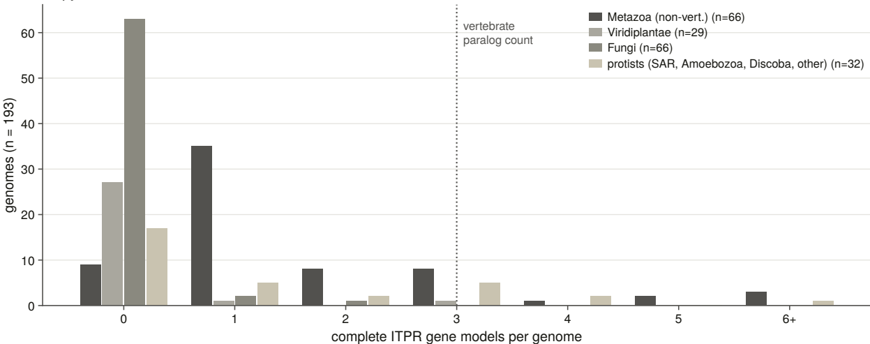
Copy number varies outside the vertebrates
