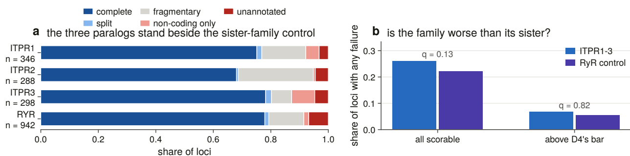
Figure 13.3. The family fails at the rate its sister family fails at in the same assemblies. Panel a stacks the five locus states for each of the three paralogs and for the ryanodine-receptor control, and panel b compares the share of loci with any failure between the family and its sister, over every scorable locus and again above the contiguity bar, with the corrected p-value printed over each pair. This comparison is what turns a failure rate into a statement about this family. The audit was built expecting a large, many-exon gene with a confusable sister family to be recorded badly, and the sister, through the same pipelines, fails at a comparable rate, so a quarter of loci not delivered as one model reads as the failure rate for vertebrate genes of this size rather than as an indictment of this family.
