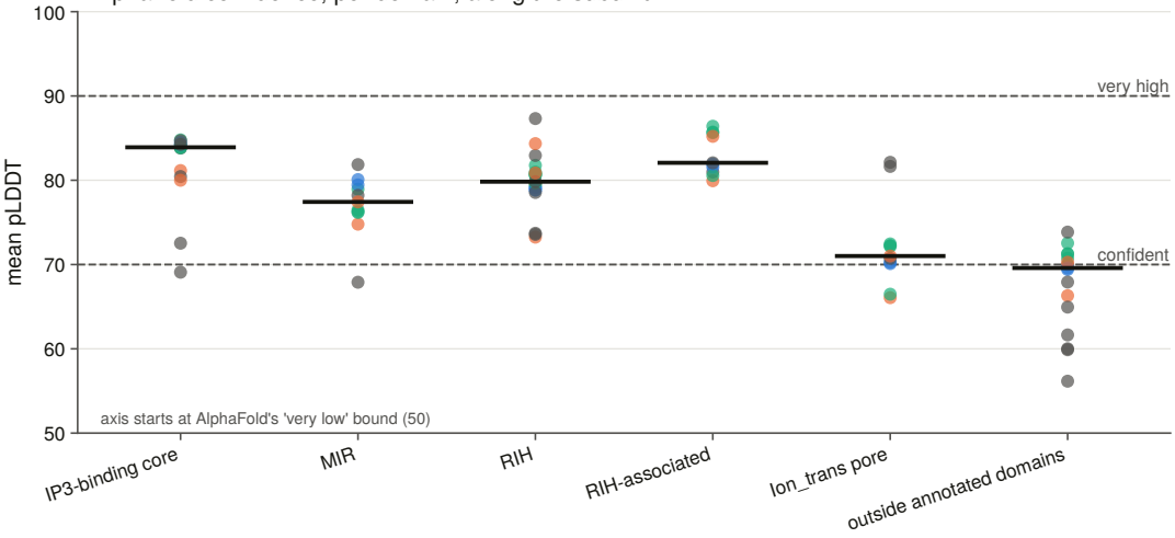
AlphaFold confidence, per domain, along the subunit
