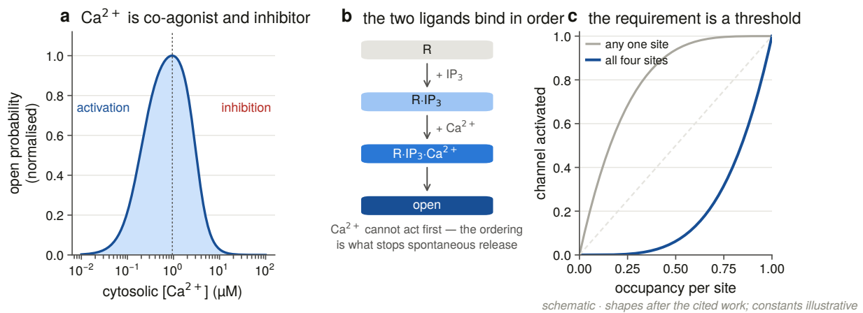
Figure 4. The three properties that make this a detector rather than a valve. (a) The bell: the same ion activates at low concentration and inhibits at high [11], so open probability is a band, not a threshold. (b) The two ligands bind in a fixed order — IP 3 first, Ca 2+ second [38] — which is why a rise in cytosolic Ca 2+ alone does not open the channel. (c) Requiring all four sites [43] turns a graded input into a switch: at 50% site occupancy, a channel needing one site is 94% activated and a channel needing four is 6%. The curves are drawn to the shape of the cited results with illustrative constants; they are not digitised data.
