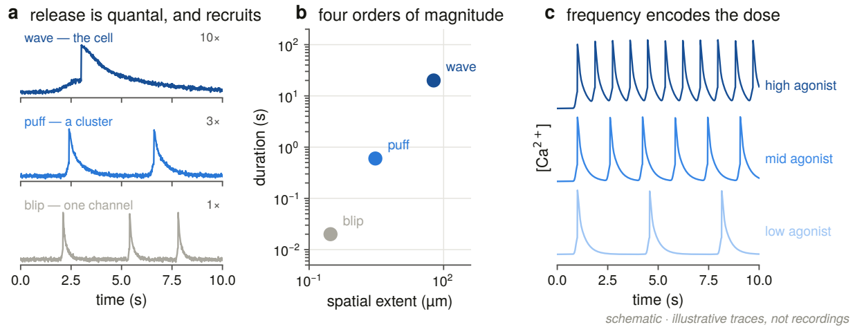
Figure 6. The signal is built, not switched on. (a) The three event classes, each on its own scale — a single channel’s blip, a cluster’s puff, and the cell-wide wave that recruitment produces [70,12]; the amplitudes differ about tenfold, so they are drawn in separate bands rather than on one axis. (b) The same three events placed by extent and duration: four orders of magnitude separate the smallest from the largest. (c) Raising agonist raises the frequency of spikes more than their size [71,72], which is what makes frequency the carried variable (§5.2). Illustrative traces, not recordings.
