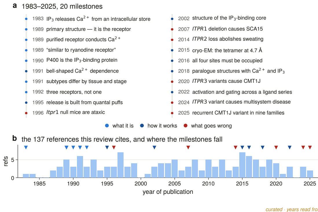
Figure 1. Four decades, and the order in which the questions were settled. (a) Twenty results that changed what the receptor was taken to be, coloured by the kind of question each answered. The resemblance to the ryanodine receptor is not a later refinement: it is in the title of one of the two 1989 cloning papers [8]. (b) The 137 references this review cites, by year, with the milestones marked — the peaks are the cloning era and the cryo-EM era. No year in this figure is transcribed; each is read from the reference table the bibliography is rendered from.
