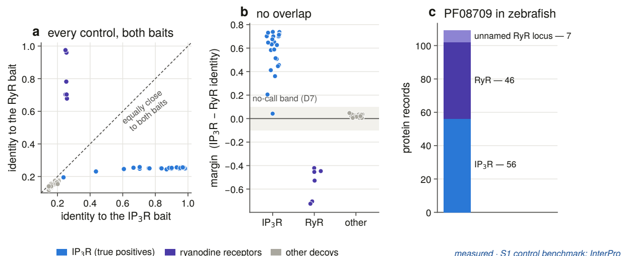
Figure 9. Separating the families by evidence rather than by name. (a) Every one of the 56 S1 controls scored against a labelled IP 3 R bait and a labelled RyR bait; the two families fall on opposite sides of the diagonal with nothing in between. (b) The same data as a margin. True IP 3 Rs run from +0.04 to +0.74 and ryanodine receptors from −0.72 to −0.44; the shaded strip is the \pm 0.10 band inside which the project declines to call either way, and the one positive sitting in it is Dictyostelium iplA. No gene symbol is consulted anywhere in this test. (c) Why it is needed: a single query for the IP 3 -binding-core domain in zebrafish returns 109 protein records, of which 53 are ryanodine receptors — including seven from an unnamed 4,900-residue locus.
