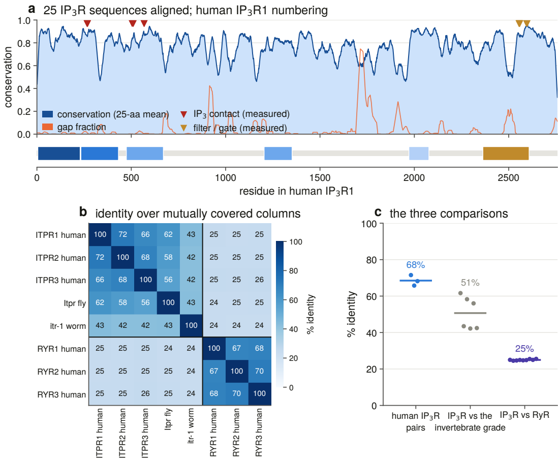
Figure 8. Constraint across the family, and how far apart its members actually are. (a) Per-column conservation from an alignment of the 25 control positives — IP 3 R1/2/3 across a vertebrate panel plus the invertebrate and non-metazoan single- itpr grade — mapped onto human IP 3 R1 numbering, over that protein’s domain architecture. The ligand-contact and pore positions measured in Figure 3 are marked; both sit on conservation maxima. The gap trace shows where the alignment is carrying indels, and the deepest troughs are the linkers between domains rather than the domains themselves. (b, c) All-pairs identity over mutually covered columns. The three human paralogues are 66–72% identical to each other and about 25% identical to a ryanodine receptor — and the fly receptor is closer to human IP 3 R1 (62%) than any IP 3 R is to any RyR. Parologue identity is high enough that the differences of §6.2 are differences of tuning, not of kind.
