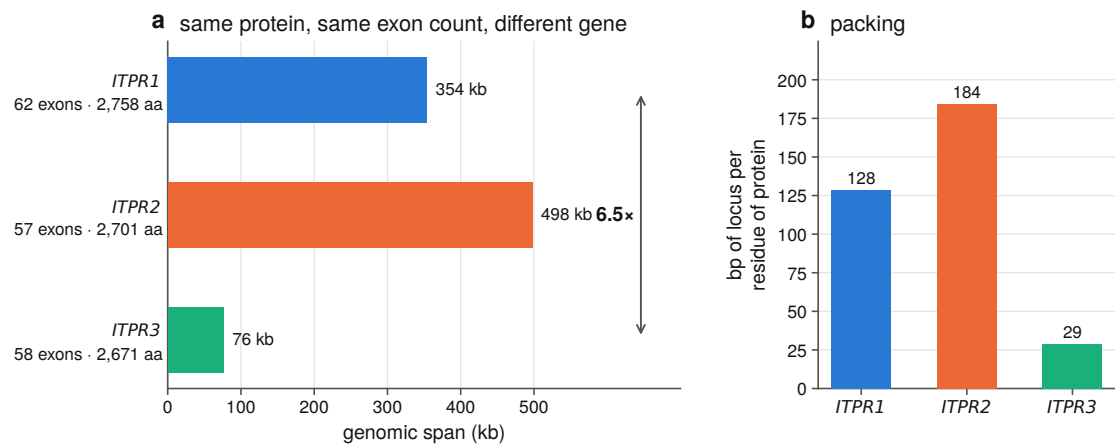
Figure 7. Three genes that make near-identical proteins out of very different amounts of DNA. (a) Genomic span; the exon count and protein length that stay constant are printed with each gene. (b) The asymmetry as one number: ITPR2 spends 184 bp of locus per residue of protein and ITPR3 spends 29. Re-derived from Ensembl release 15.12 for this review — the claim this replaced, that all three span “hundreds of kb”, is one of the four that failed audit (§12.2).
