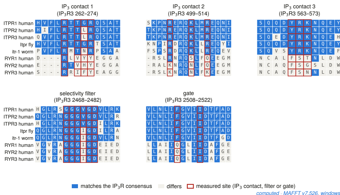
Figure 10. Where the two families agree, and where they stop agreeing. Five windows of a MAFFT alignment of both families, each anchored on a site measured in the 6DQN structure (Figure 3) rather than on a residue list taken from a paper: the three stretches that contact the bound IP 3 , the selectivity filter and the gate. Cells are shaded where the residue matches the
