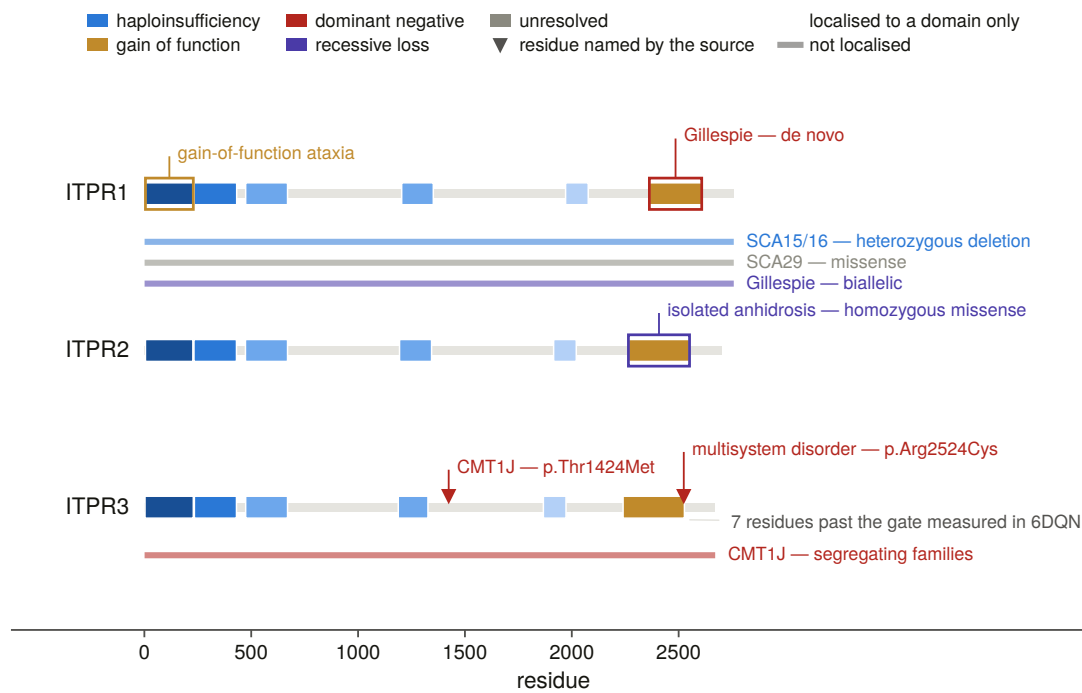
Figure 12. The clinical panel placed on the three paralogs, coloured by mechanism. The figure is drawn at the resolution the sources give, and the three resolutions are distinguished deliberately: a marker where the source names a residue, an outlined box where it localises the variant to a domain and no further, and a bar under the gene where it does neither. Read this way the panel is thinner than it looks — only two of the nine entries have a residue behind them. Both are in ITPR3 , and the recurrent multisystem variant p.Arg2524Cys sits seven residues past the gate measured in Figure 3, on the load-bearing stretch of §2.4. SCA29 is marked unresolved rather than dominant-negative: §9.1's sources establish that it is dominant and missense, and that at least one variant is a gain of function [37], which is not the same mechanism as the Gillespie and ITPR3 variants.
