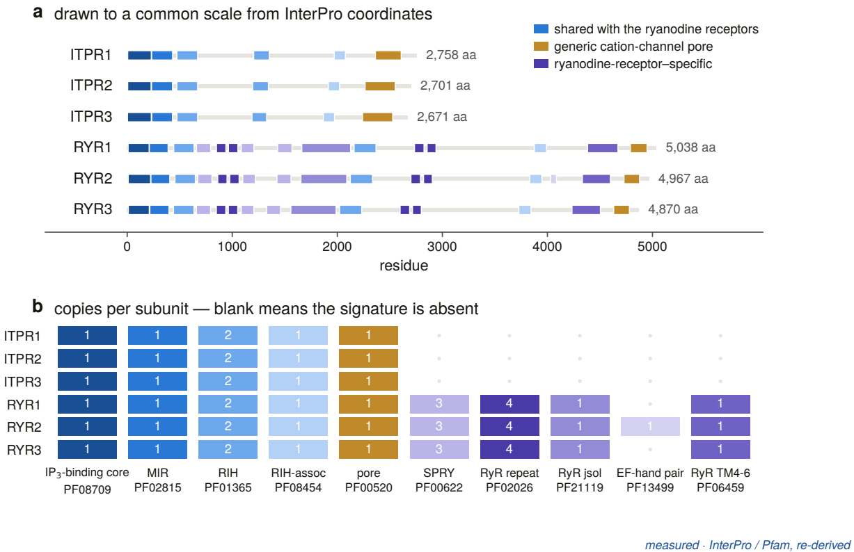
Figure 2. Every signature that defines an IP 3 receptor is also carried by a ryanodine receptor. (a) The six human proteins drawn to one scale from InterPro coordinates. (b) Copies per subunit; a blank cell means the signature is absent. The four shared signatures and the generic pore are identical in content between the families — including copy number, down to the two RIH domains. What separates them is what RyR carries in addition : four further domains and some 2,200 extra residues. A search built on the domains in the blue and amber columns cannot distinguish the two families, which is the practical form of §7.1’s argument about descent.
