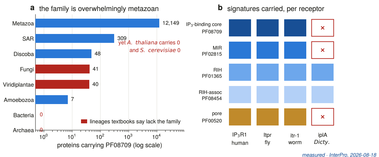
Figure 11. The signature’s reach, and its two failure directions. (a) Proteins carrying the IP 3 -binding core by lineage: 12,149 of 12,338 are metazoan, yet the set contains 41 fungal and 40 plant entries — while the reference proteomes of Arabidopsis and S. cerevisiae contain none. Either the counts are wrong or the textbooks are. (b) The opposite error, and the sharper one for a census: Dictyostelium iplA is a characterised IP 3 receptor that carries neither the IP 3 -binding core nor the MIR nor the pore domain — three of the five signatures — so an enumeration built on the family’s defining domain would not return it at all. A database count is a statement about annotation before it is a statement about genomes.
